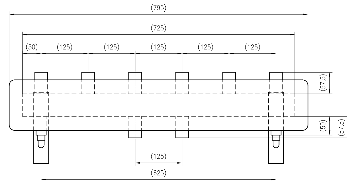
Front view
