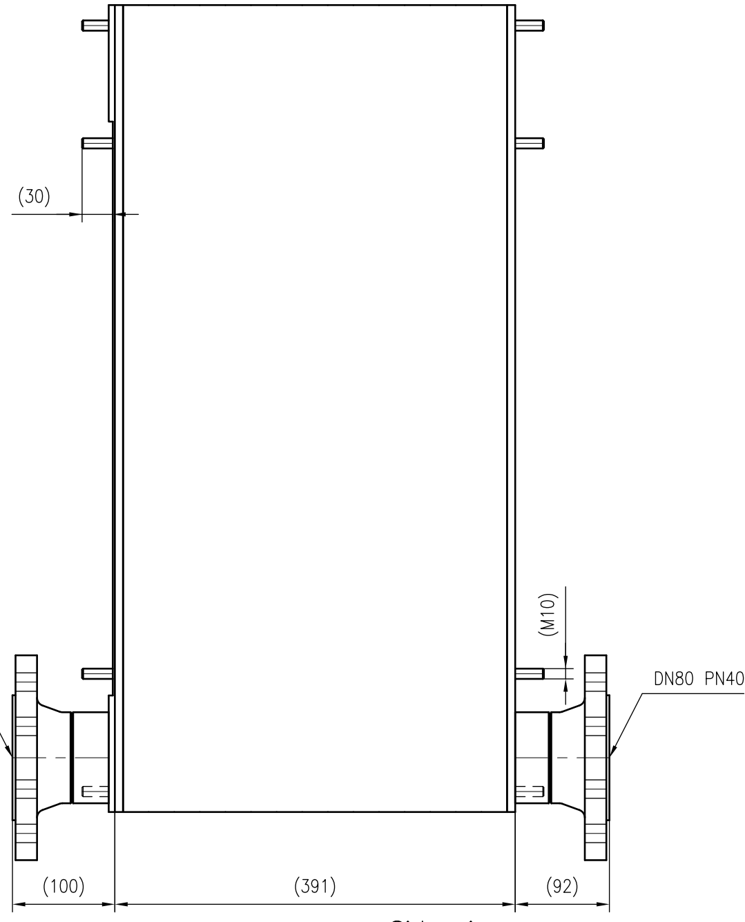
Side view
