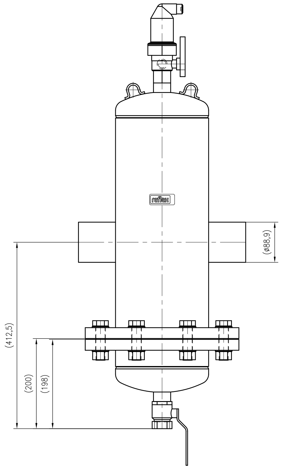
Front view
