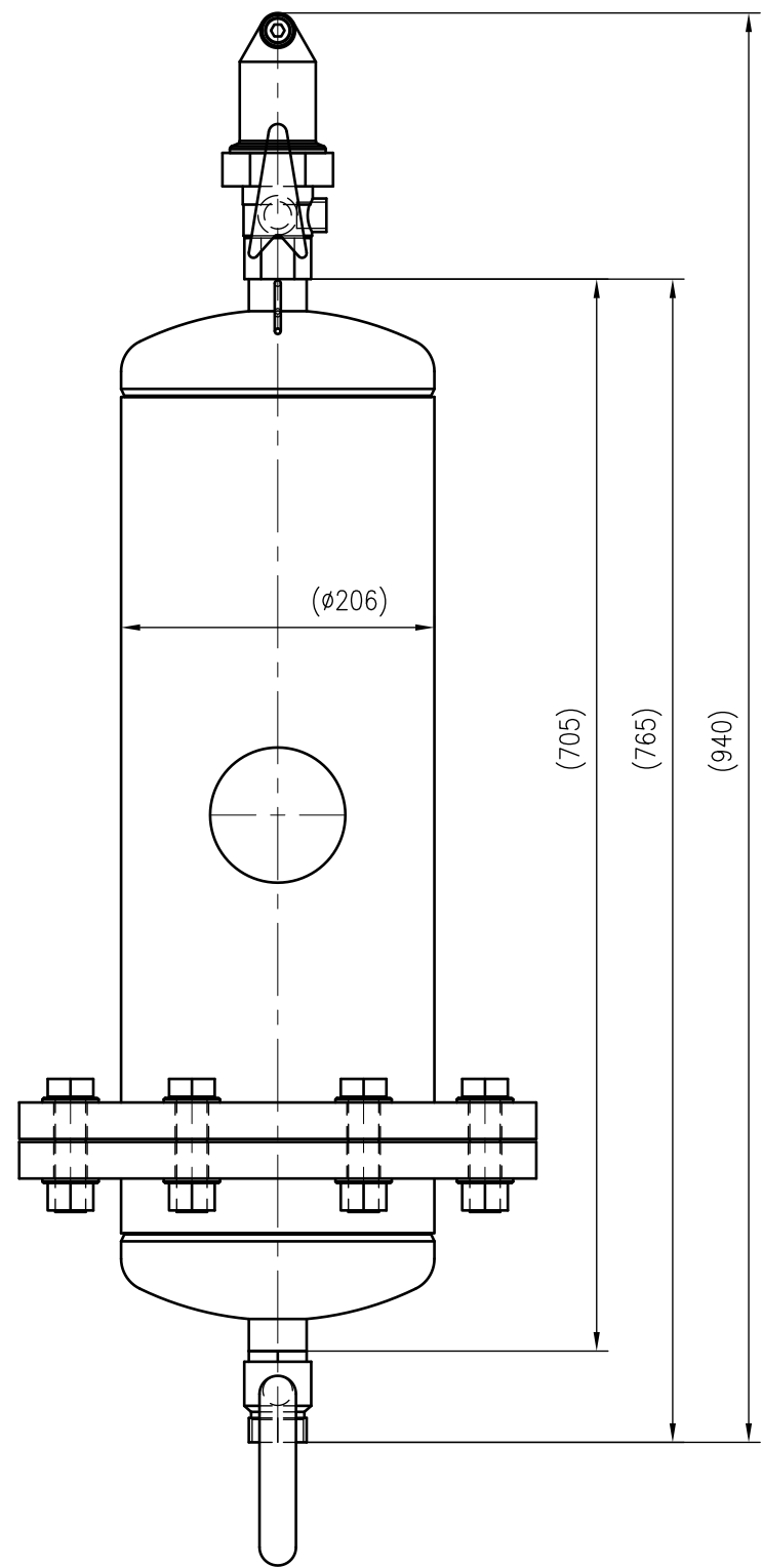
Side view
