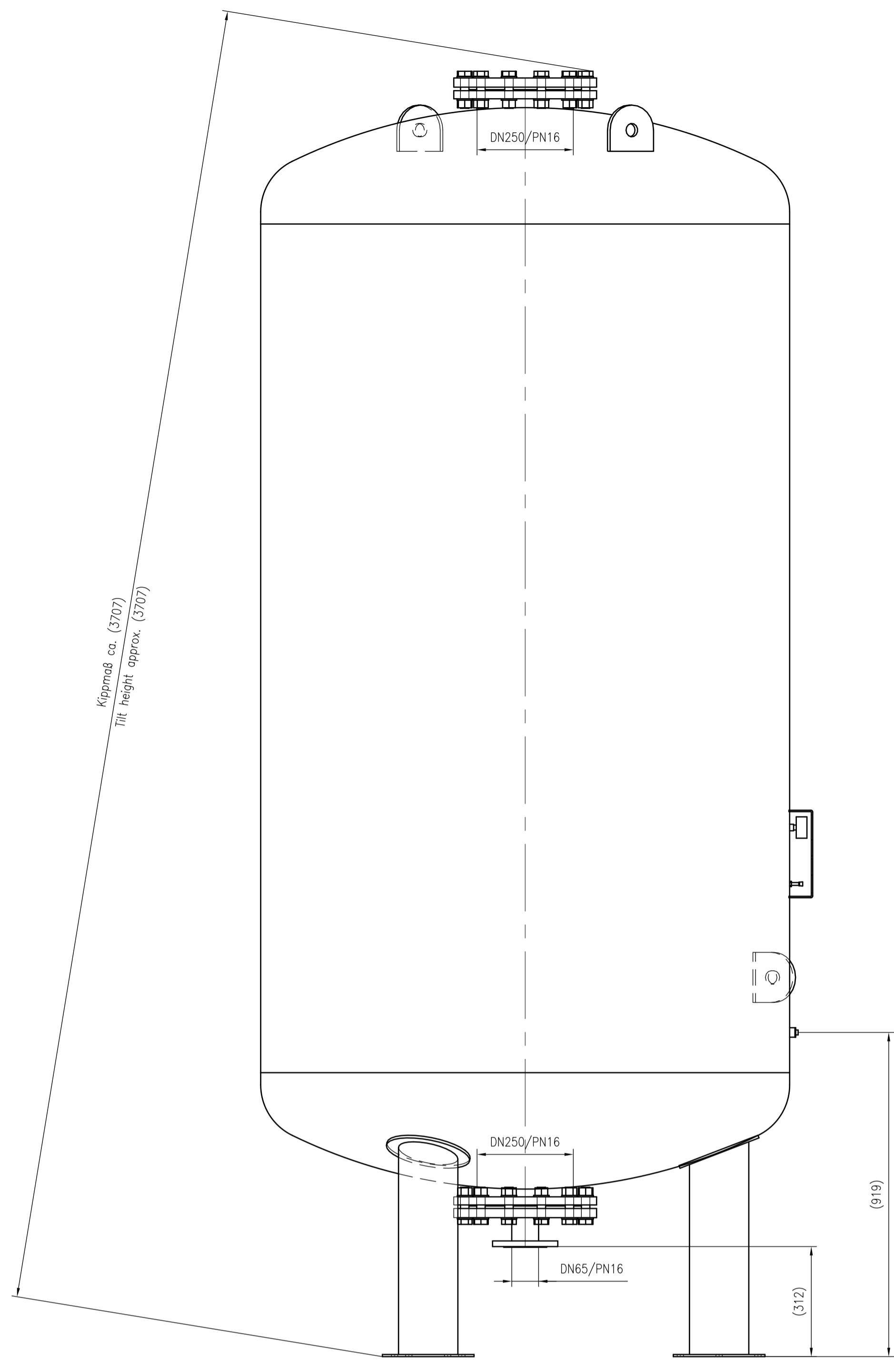
Side view
