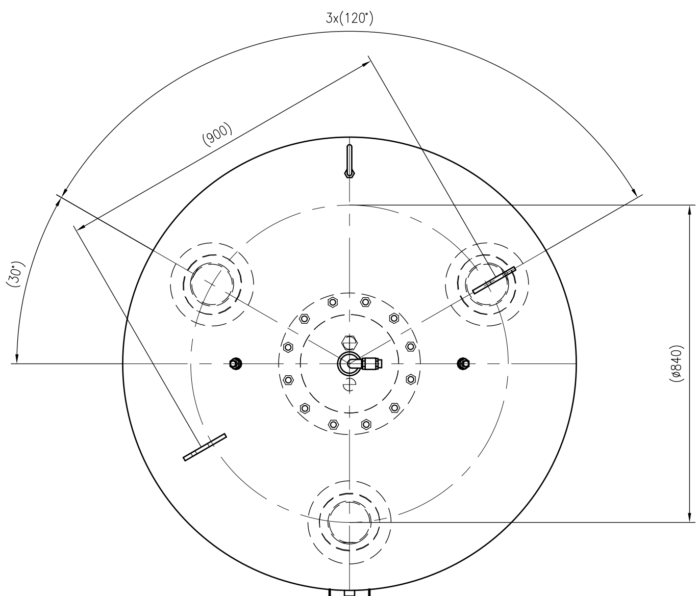
Top view
