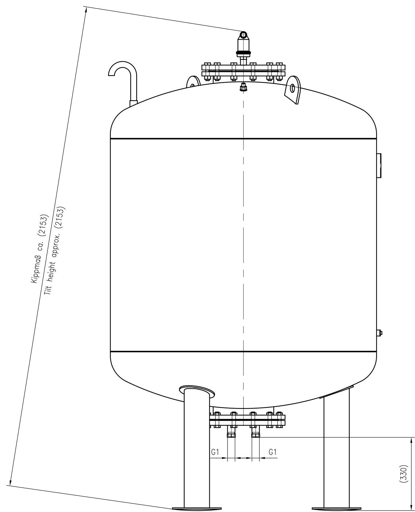
Side view
