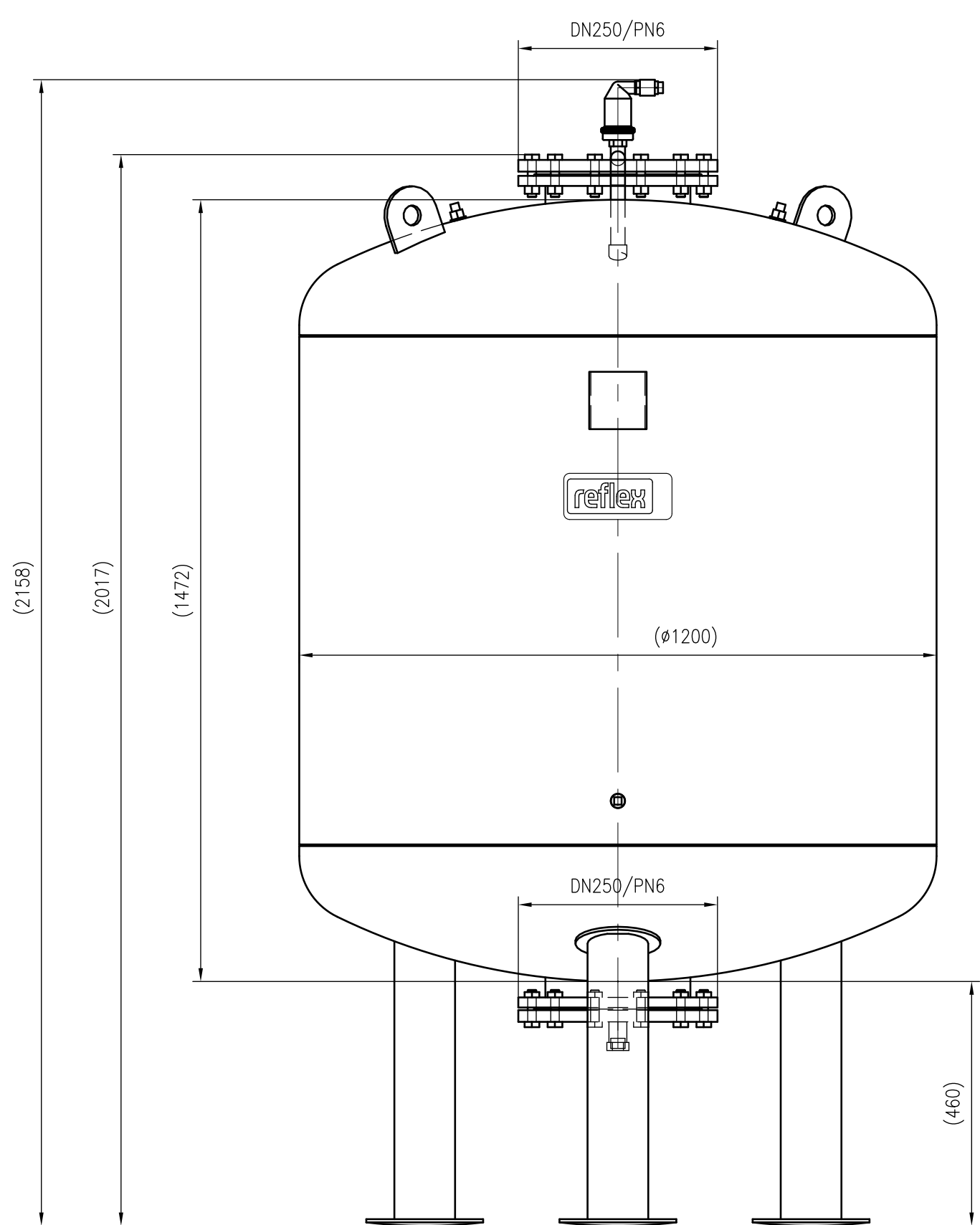
Front view
