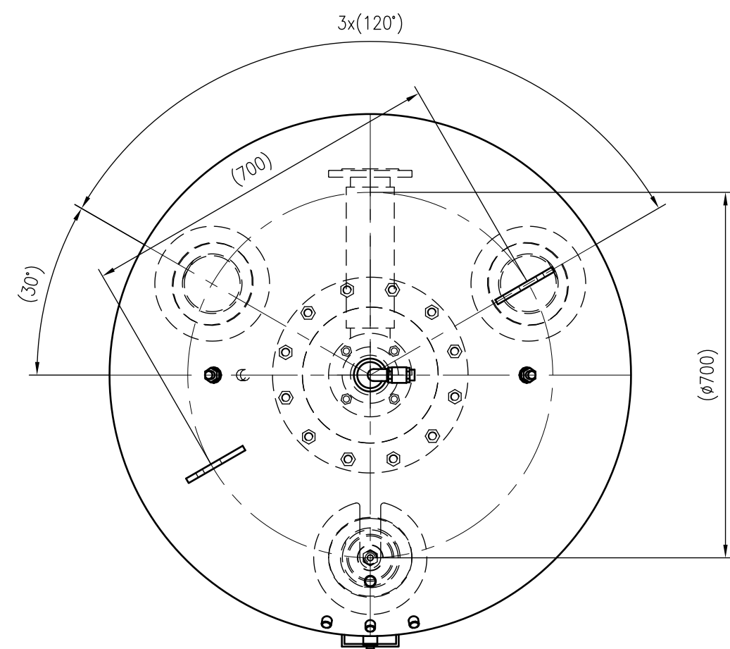
Top view
