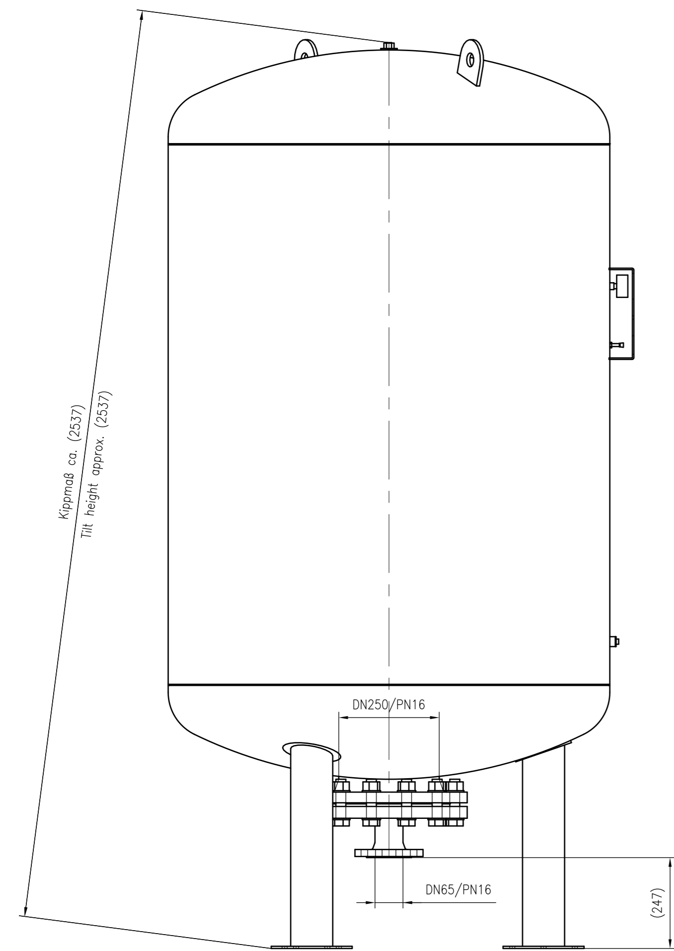
Side view
