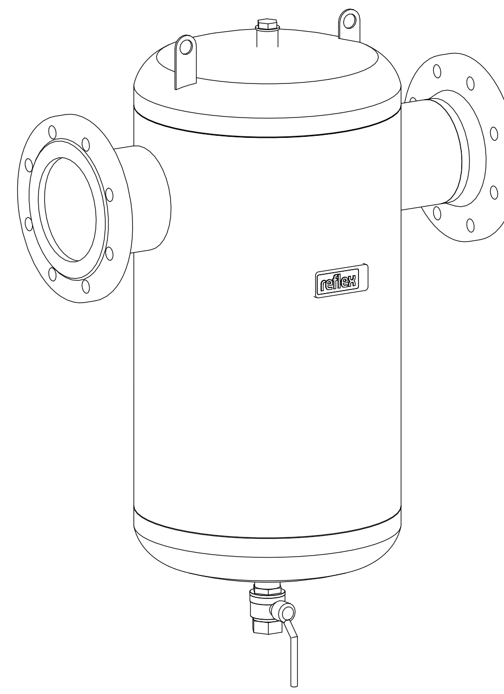
Isometric view
