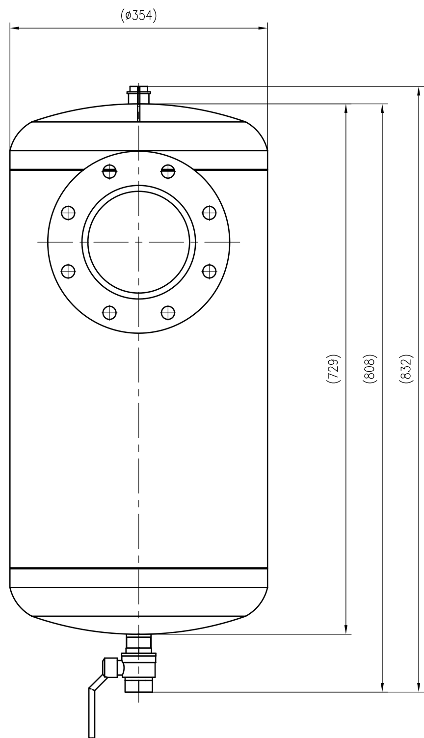
Side view
