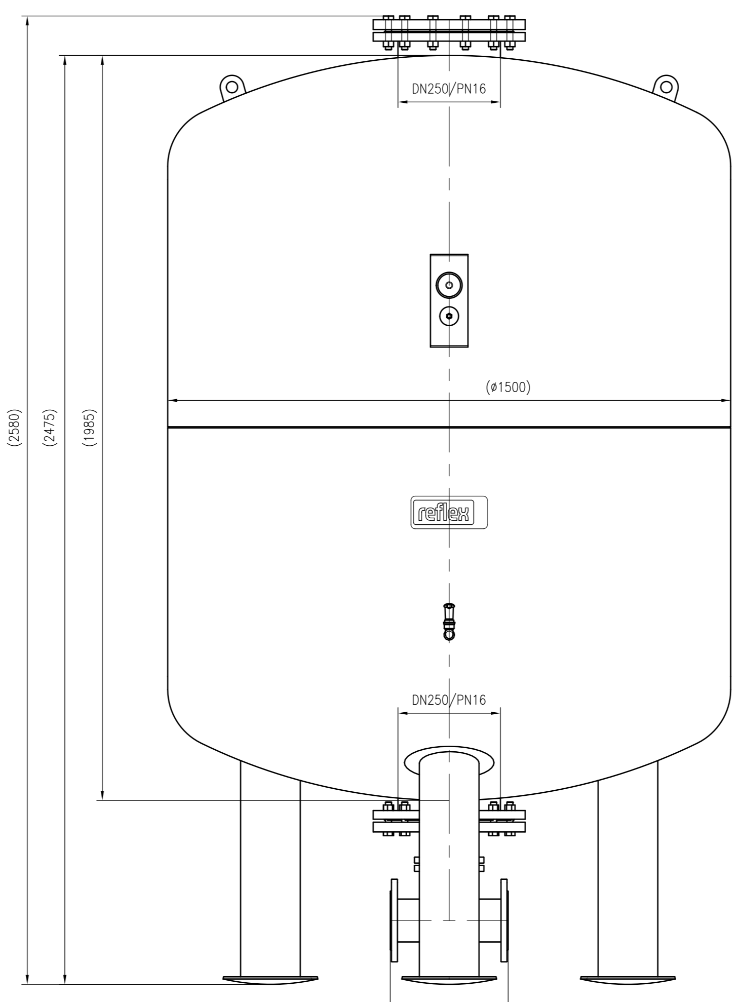
Front view
