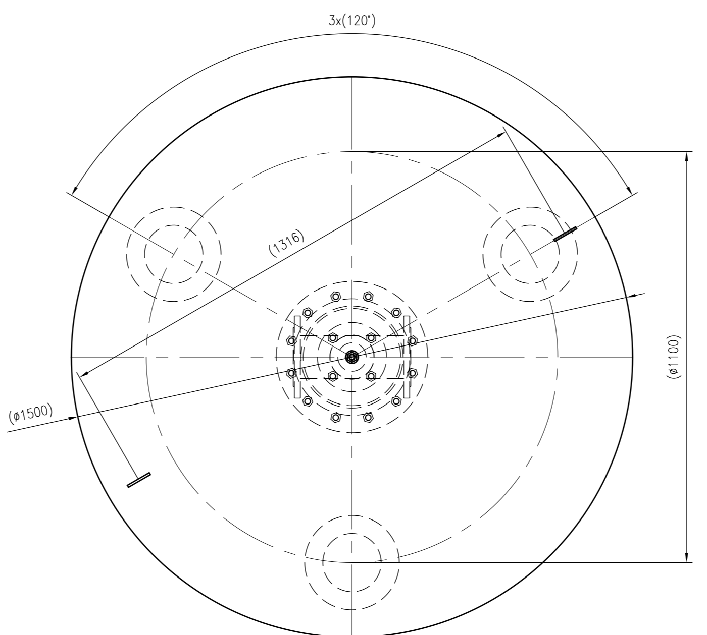
Top view
