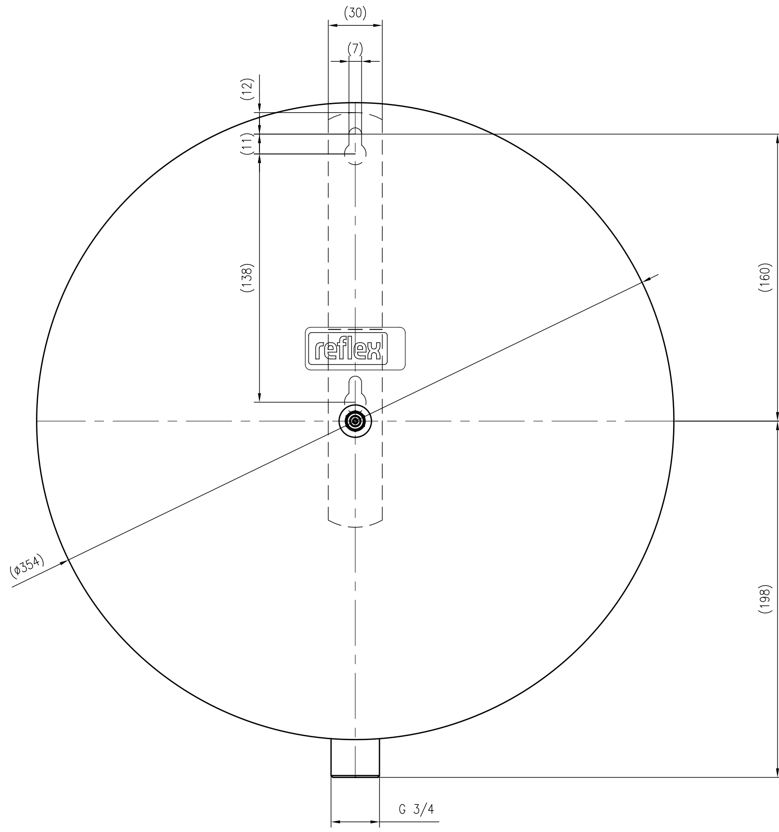
Front view
