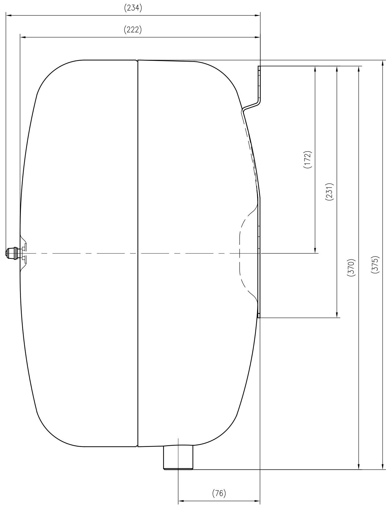
Side view
