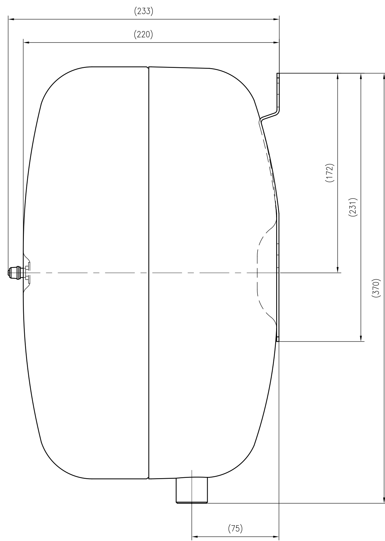
Side view
