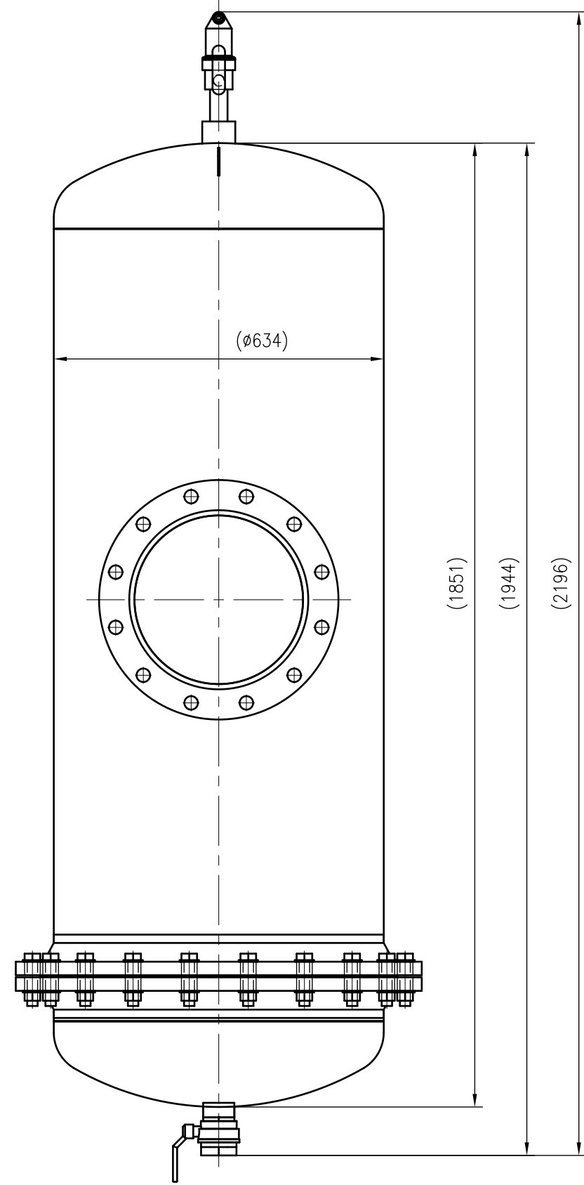
Side view
