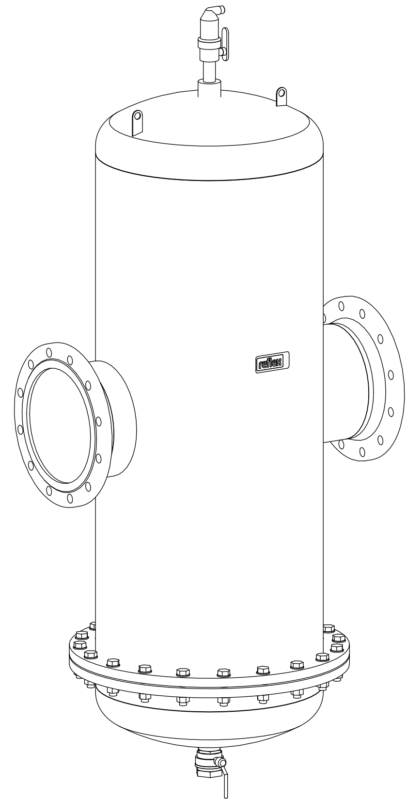
Isometric view
