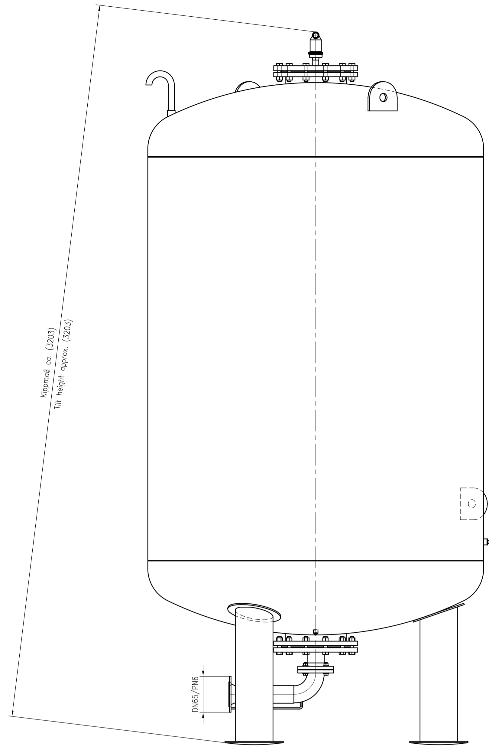
Side view
