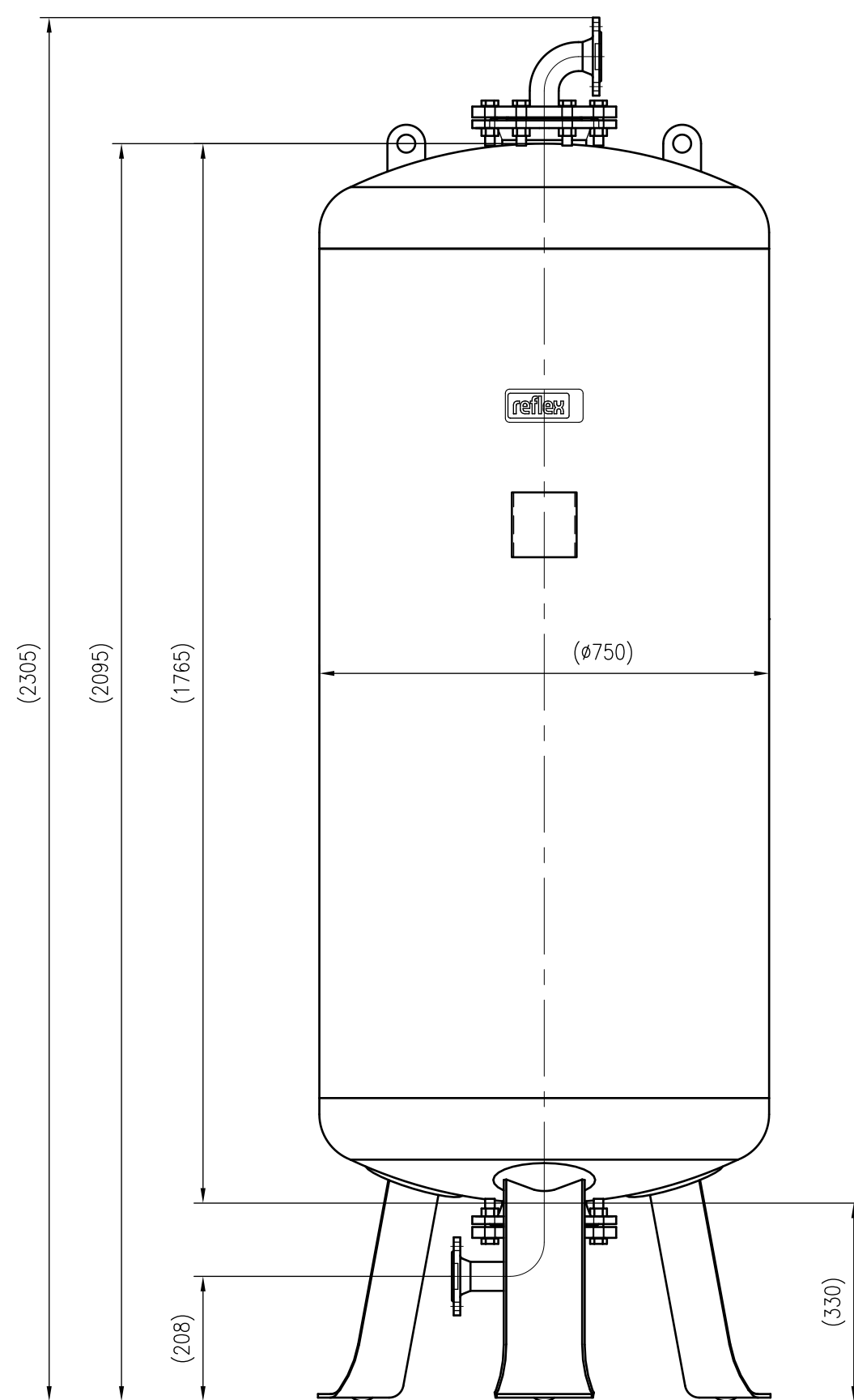
Front view
