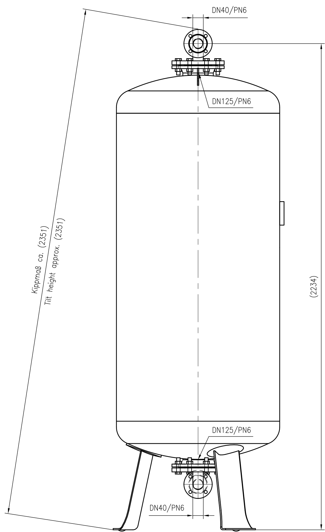
Side view
