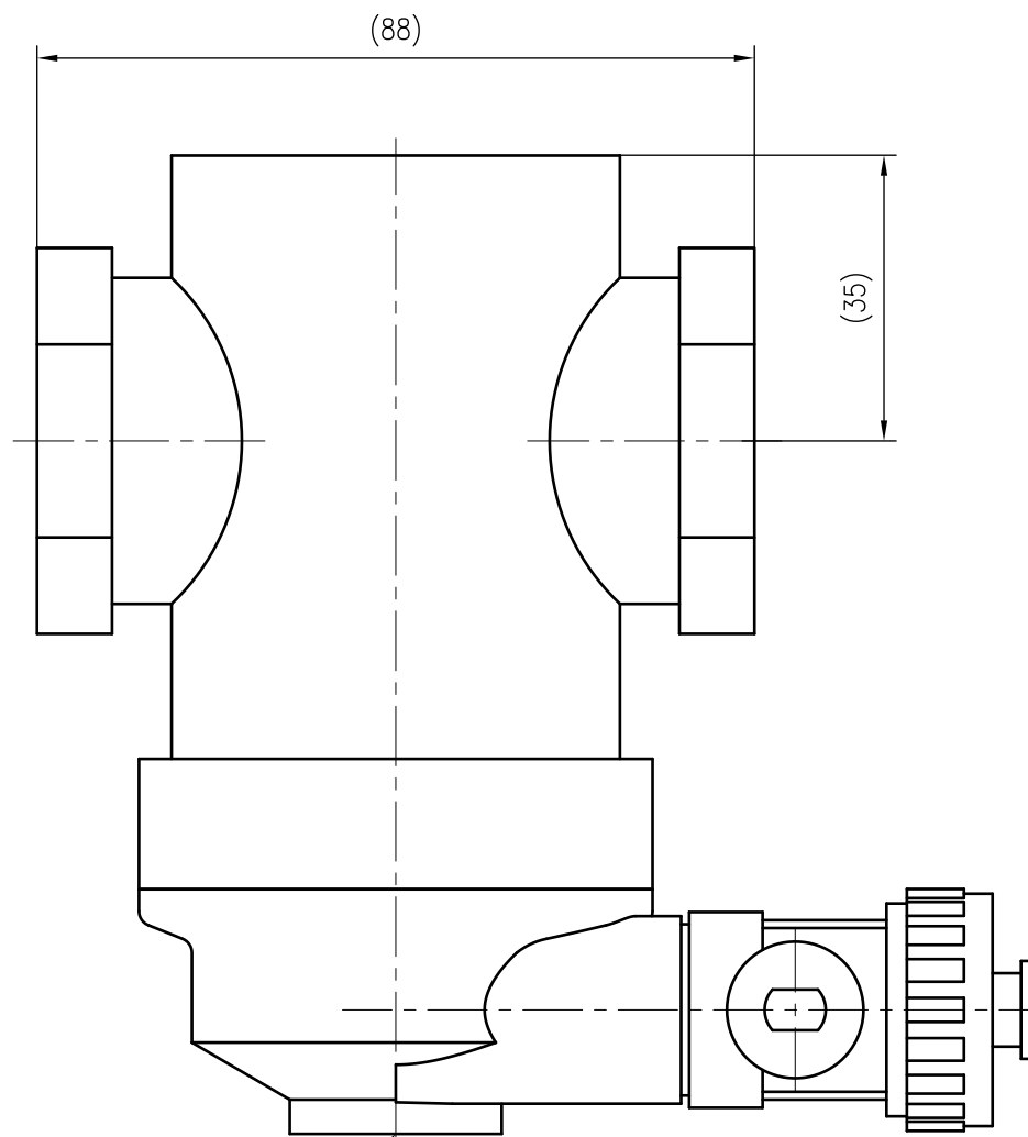
Front view
