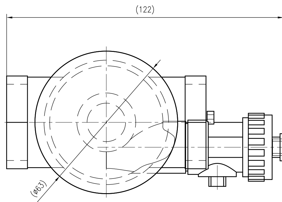
Top view
