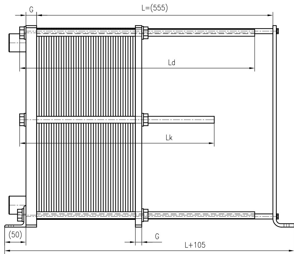
Side view
