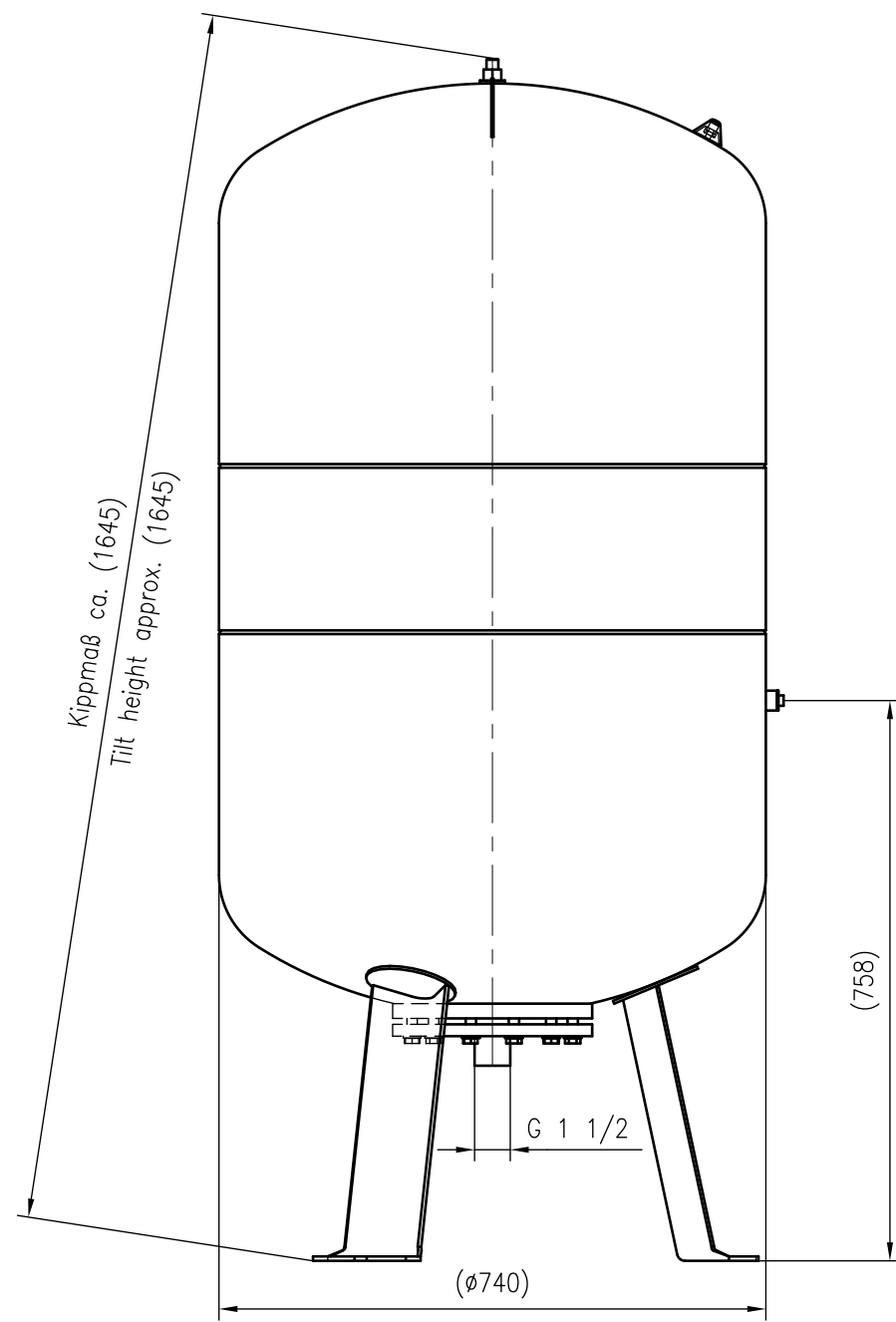
Side view
