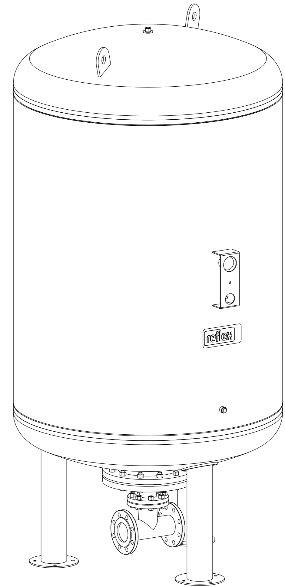
Isometric view
