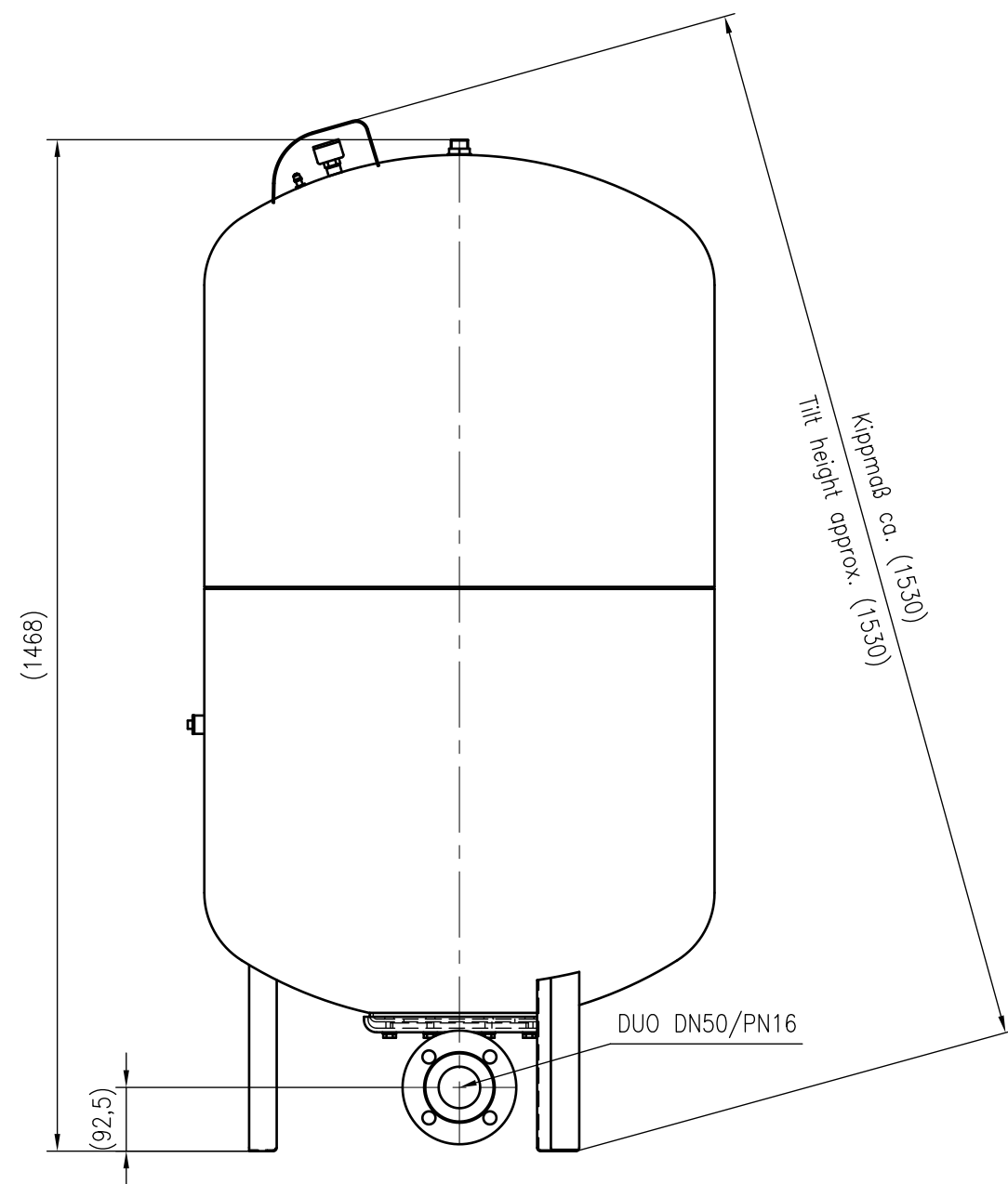
Side view
