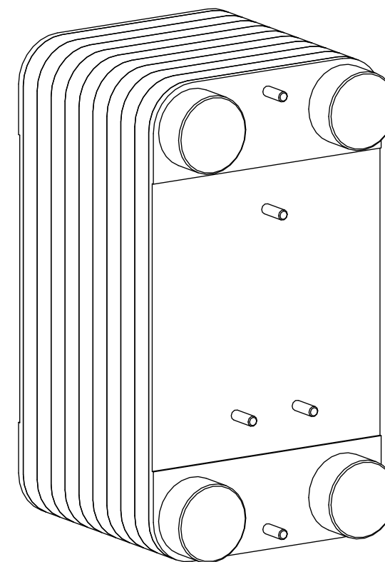
Isometric view
