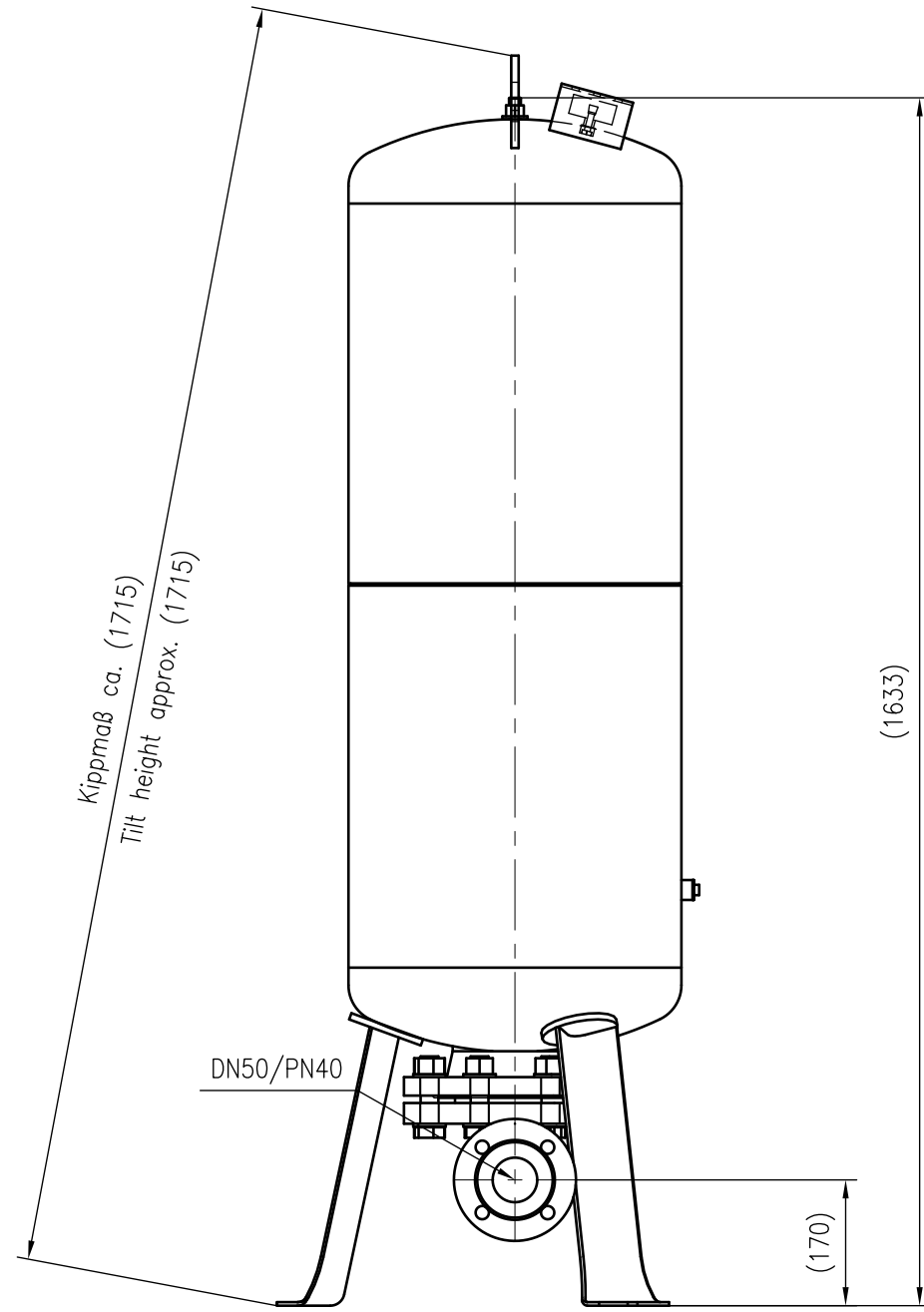
Side view
