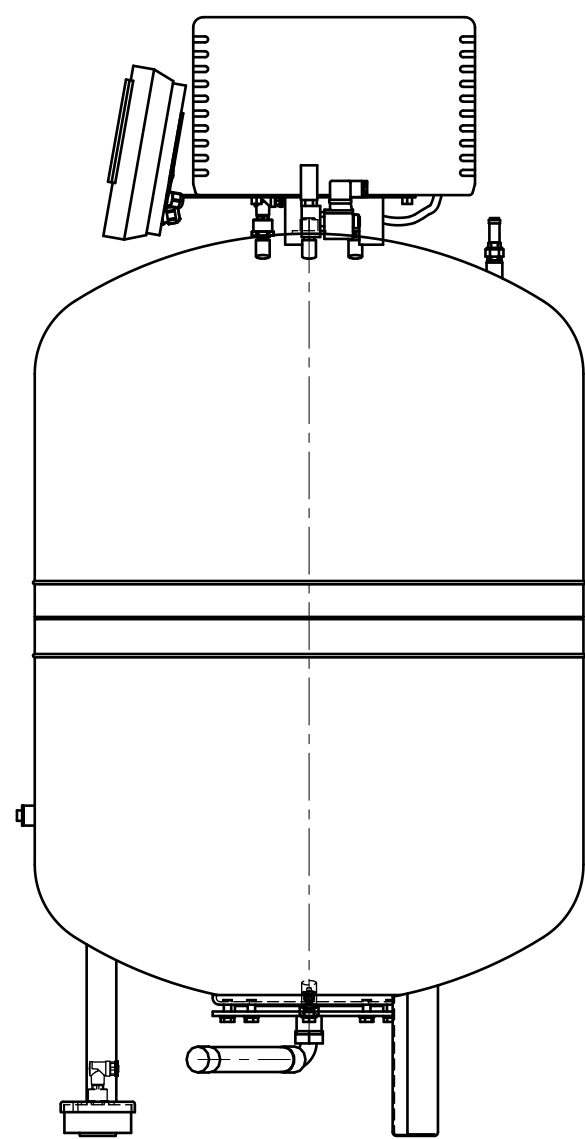
Side view
