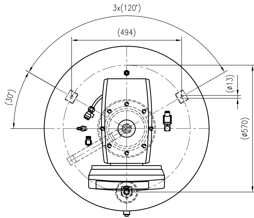
Top view
