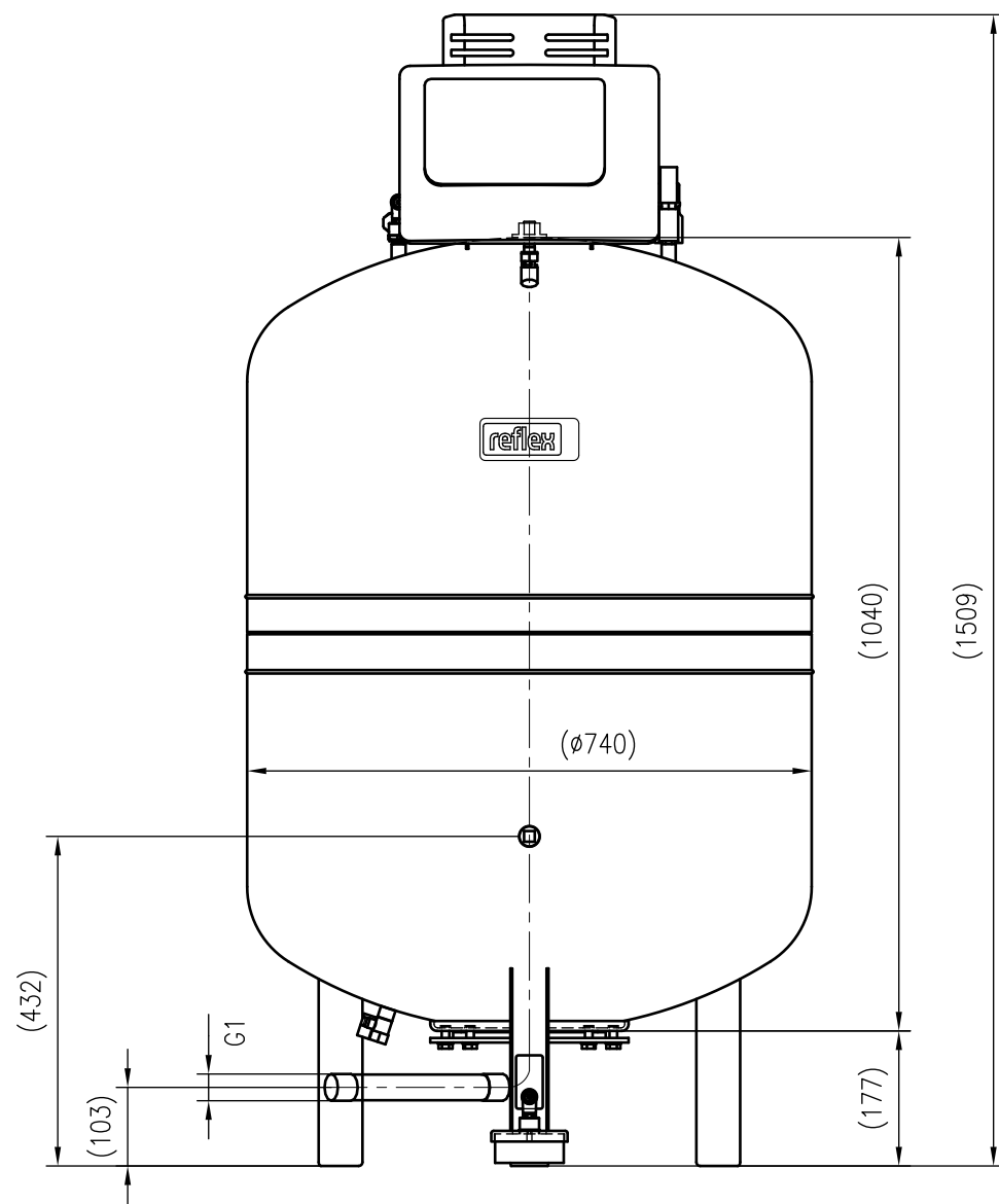
Front view
