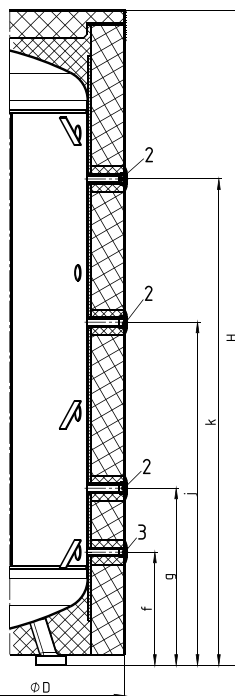
Section view B-B
