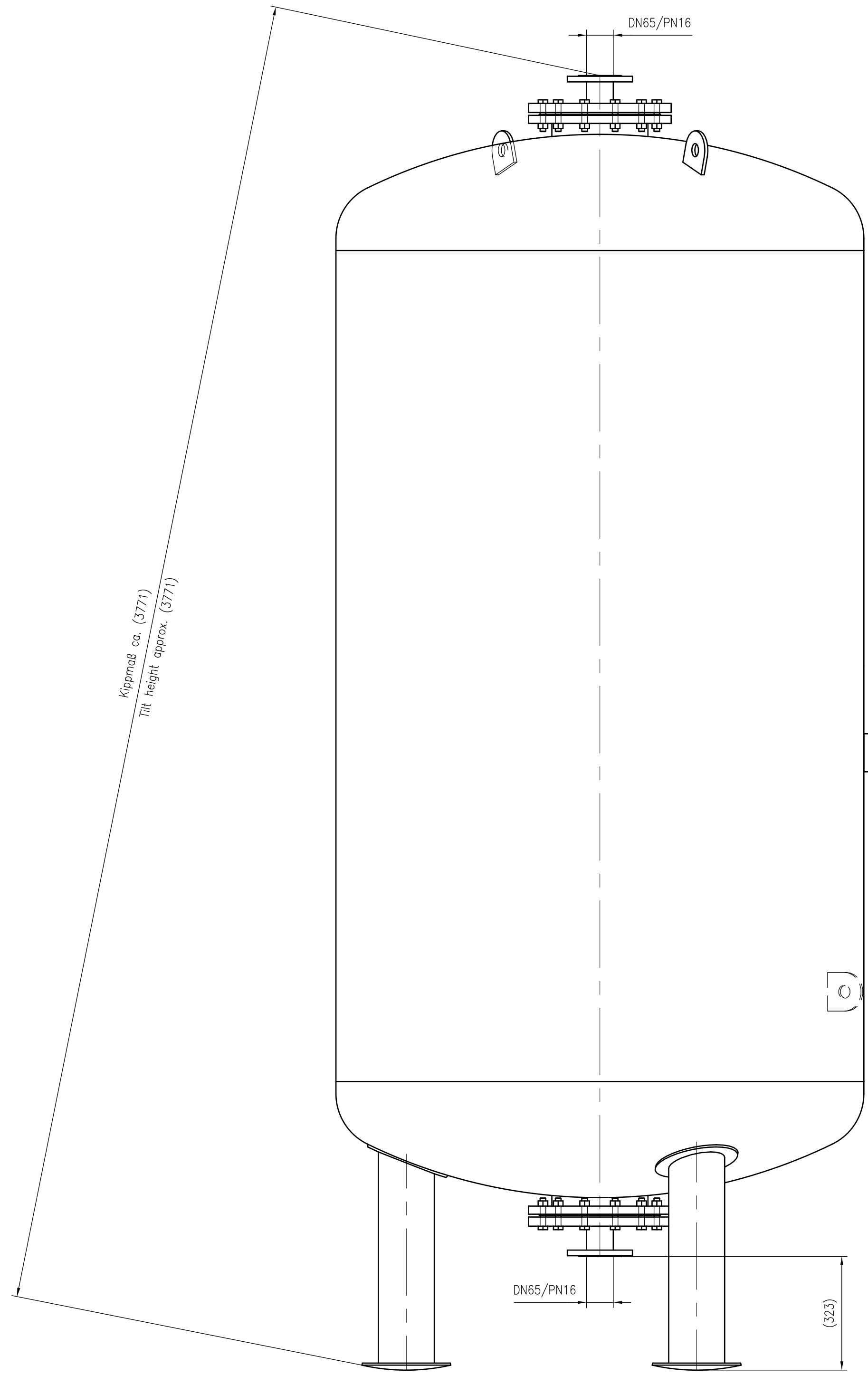
Side view
