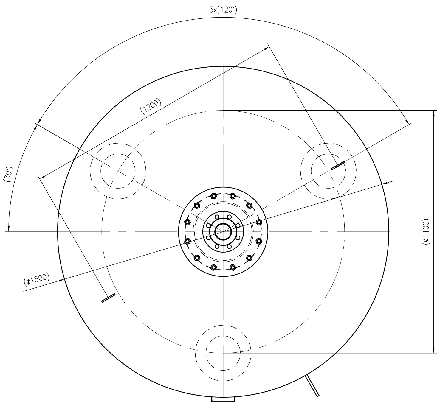
Top view
