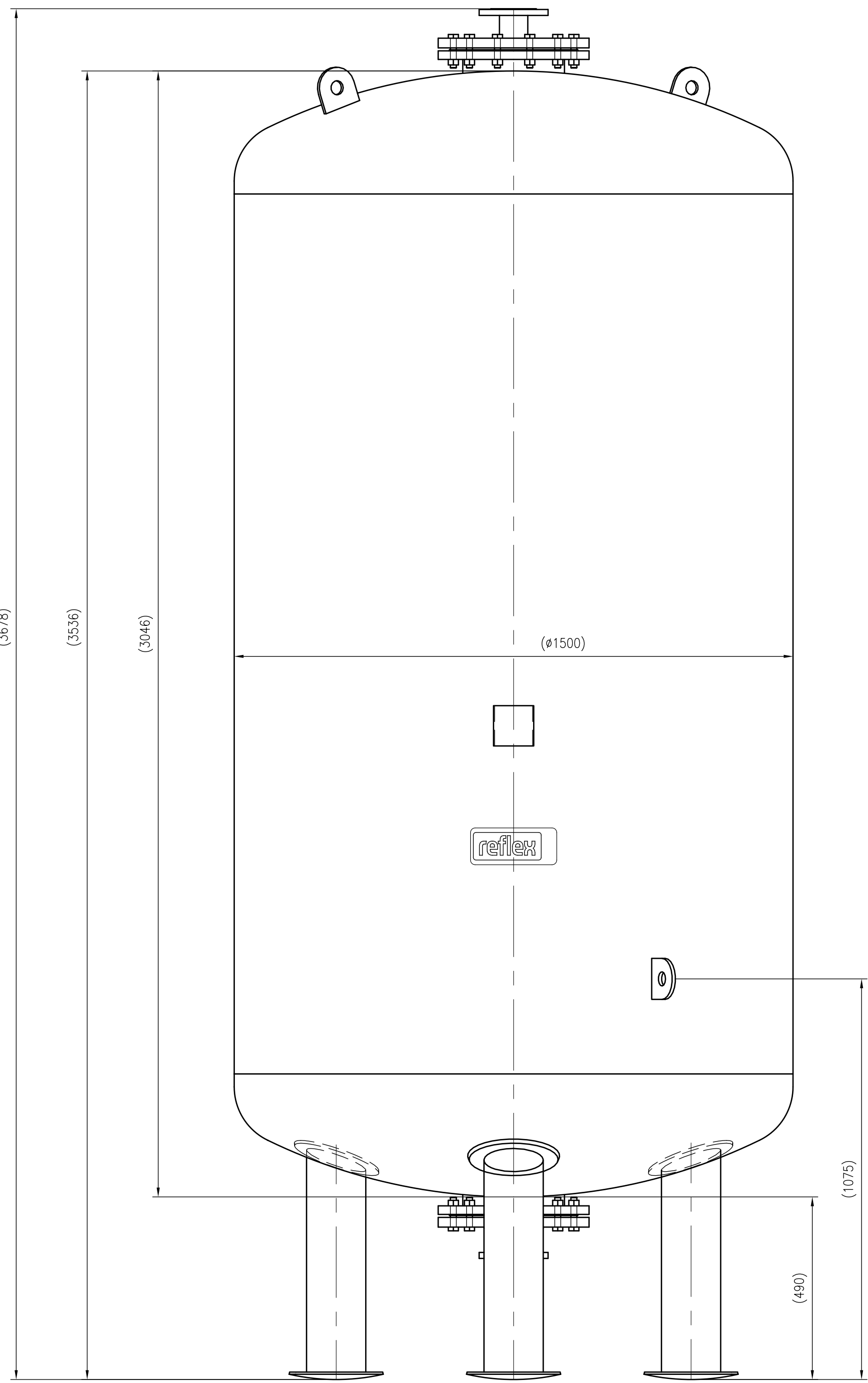
Front view
