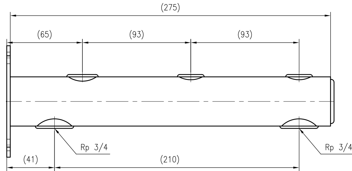
Front view
