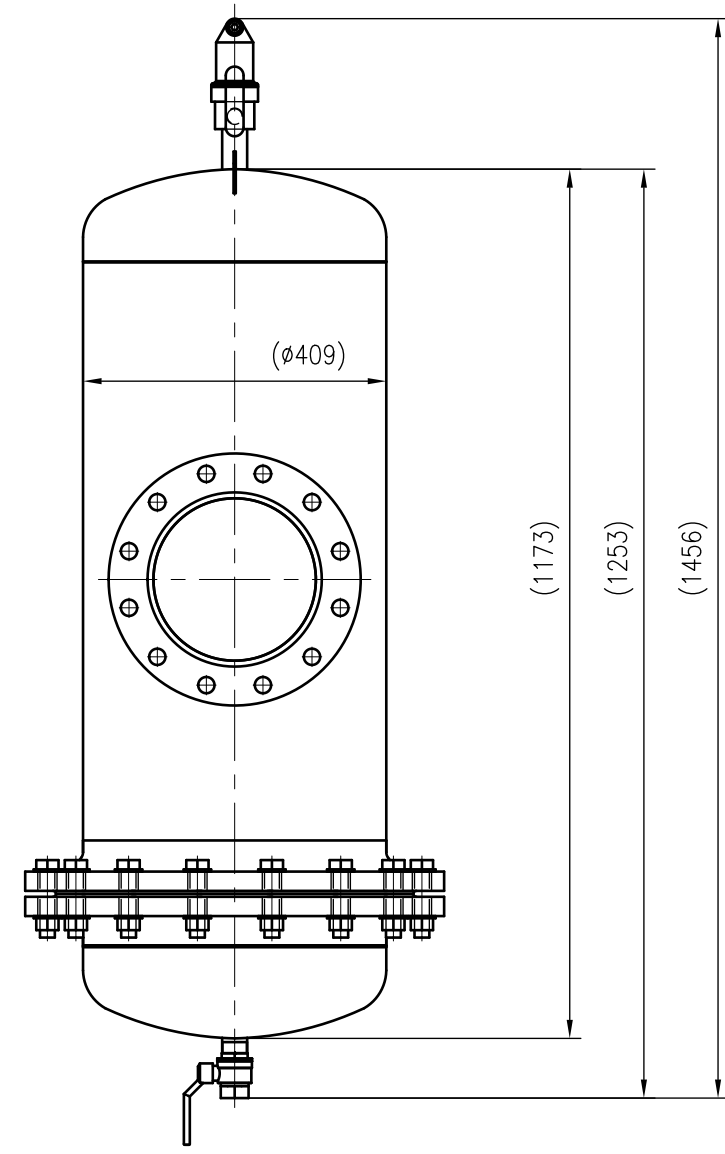
Side view
