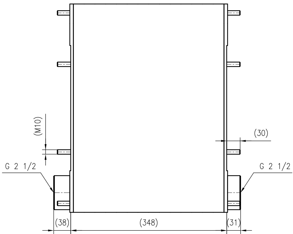
Side view
