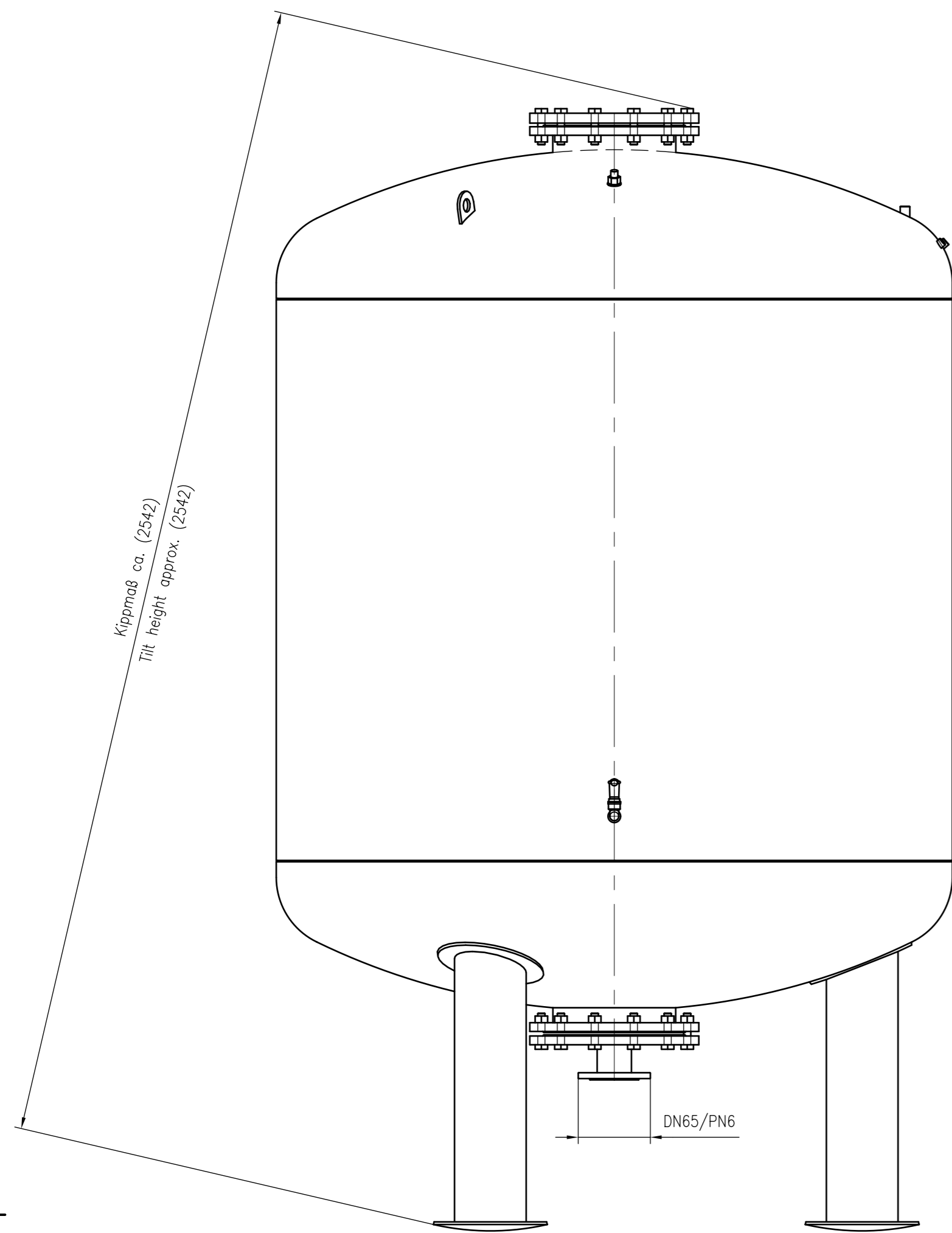
Side view
