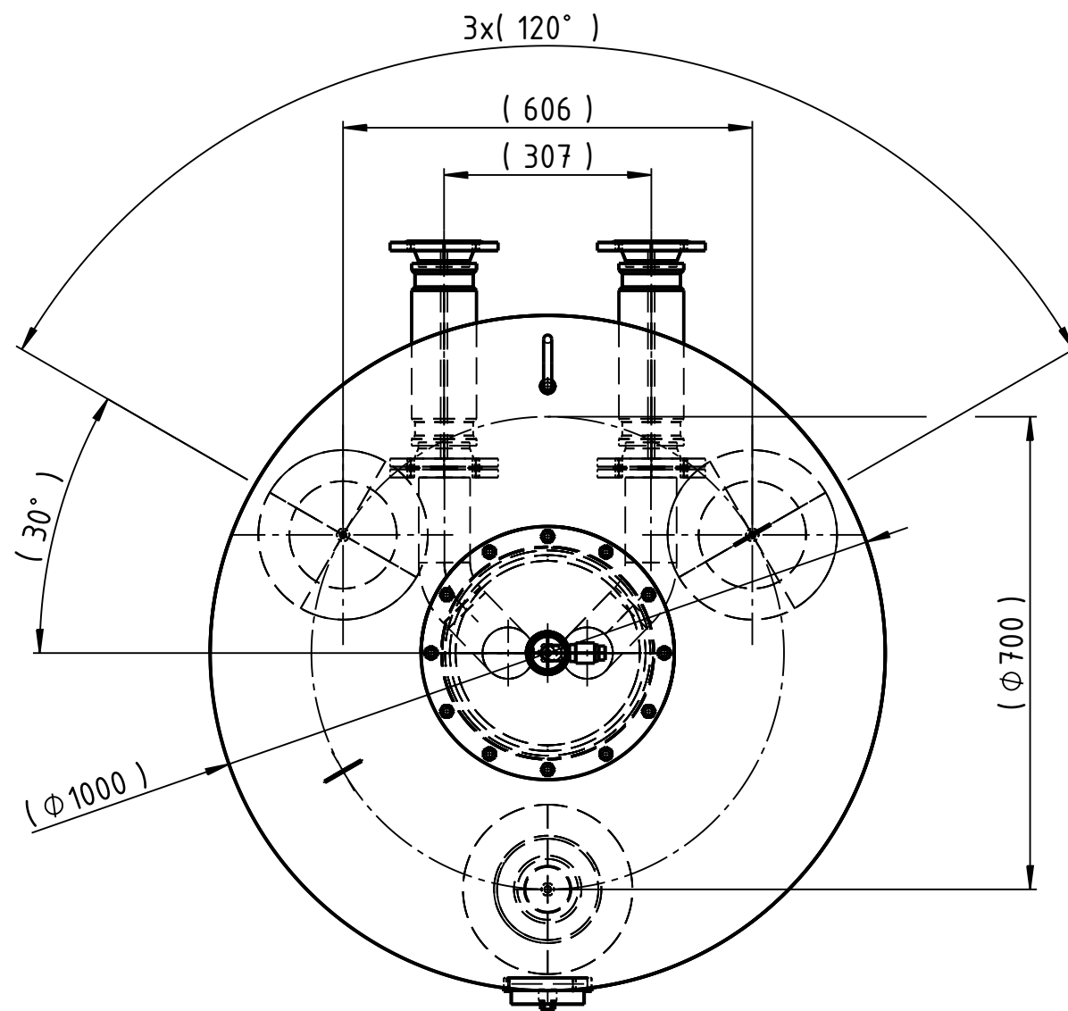
Top view
