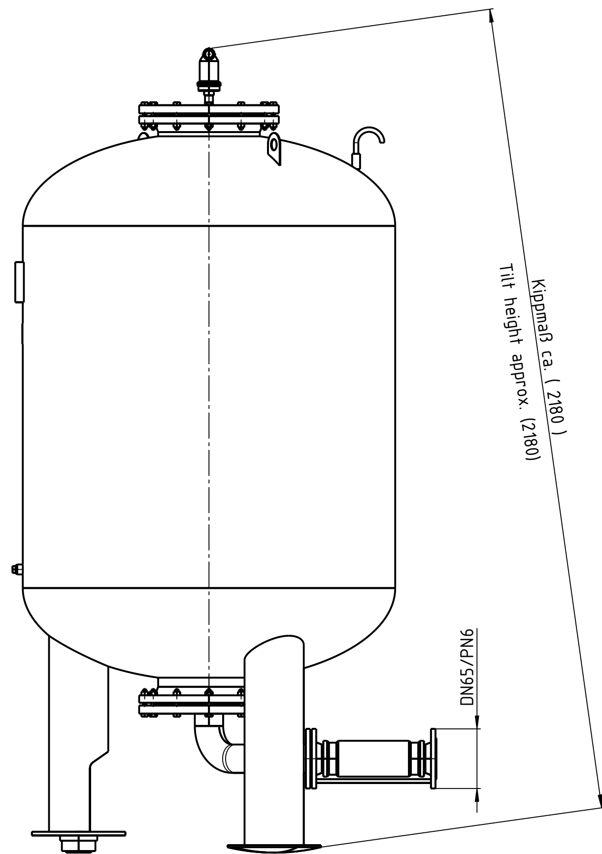
Right view
