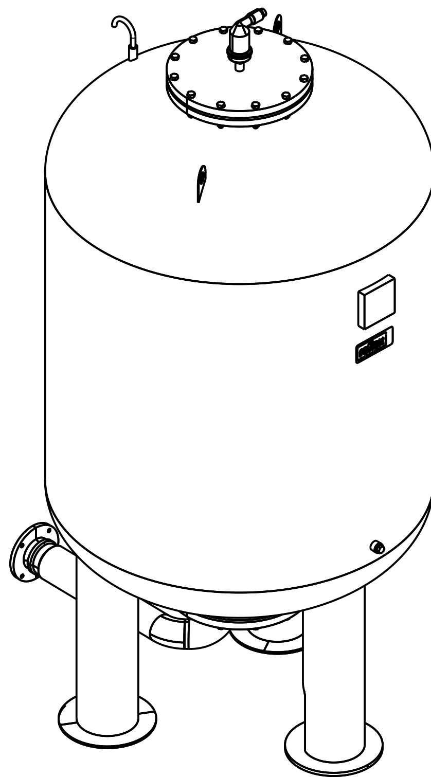
Isometric view
