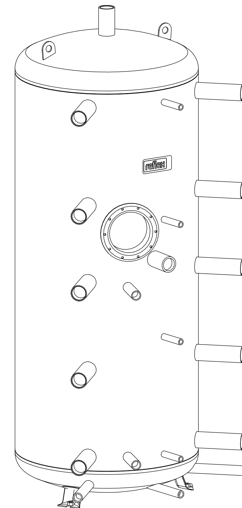
Isometric view
