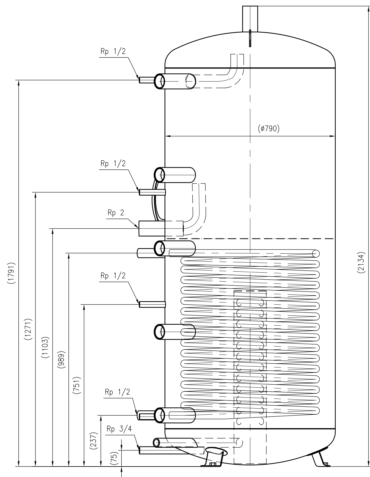
Side view
