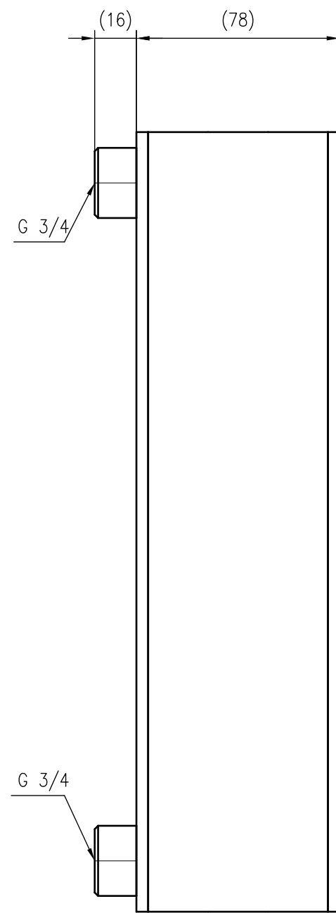
Side view
