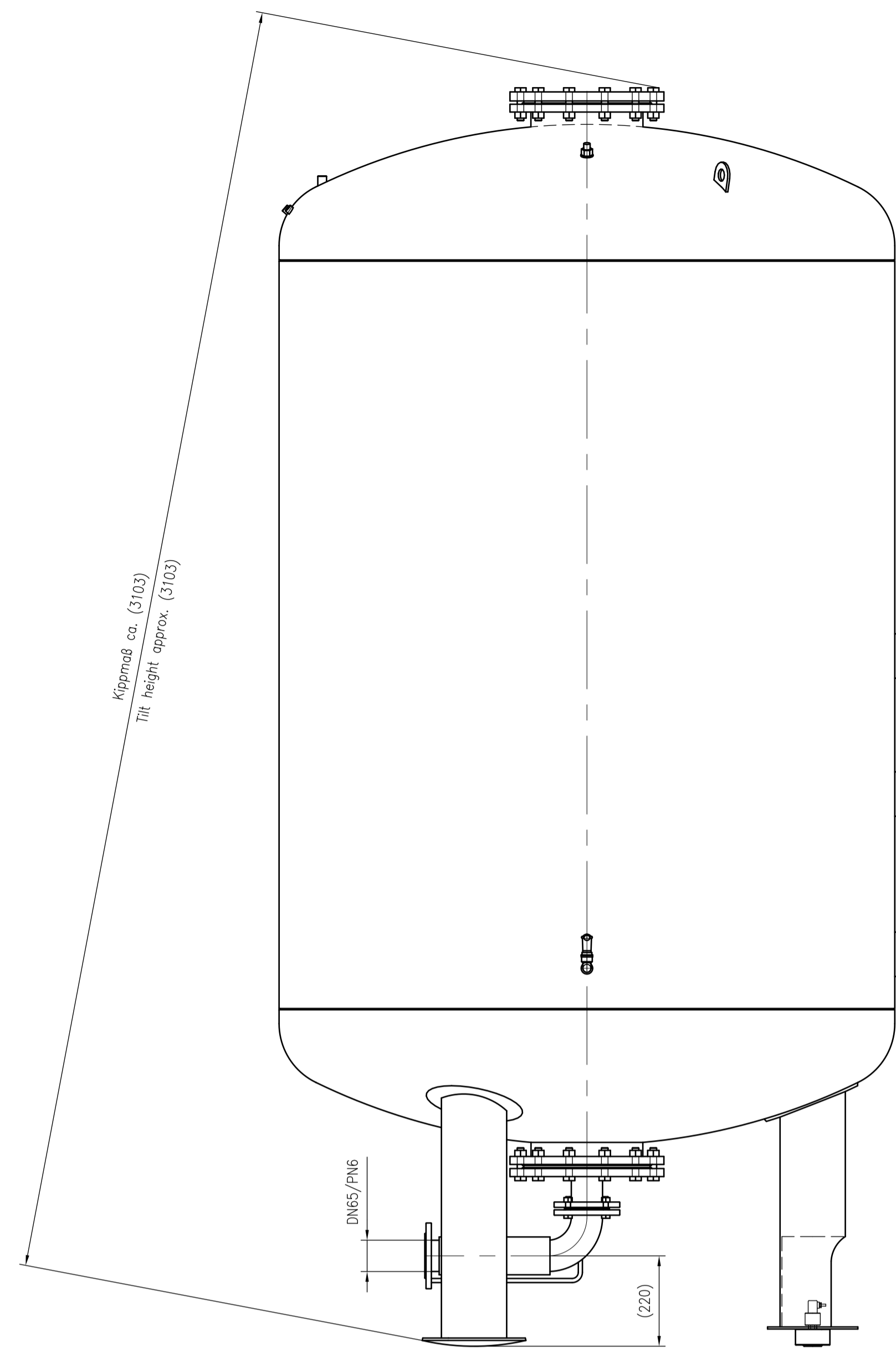
Side view
