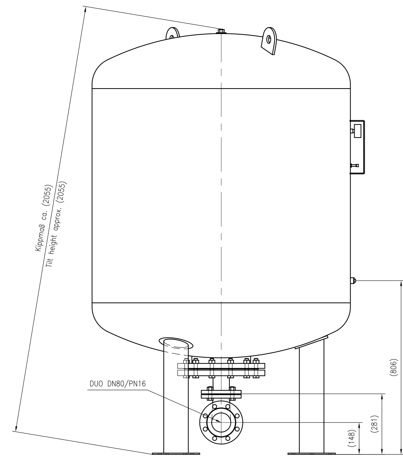
Side view
