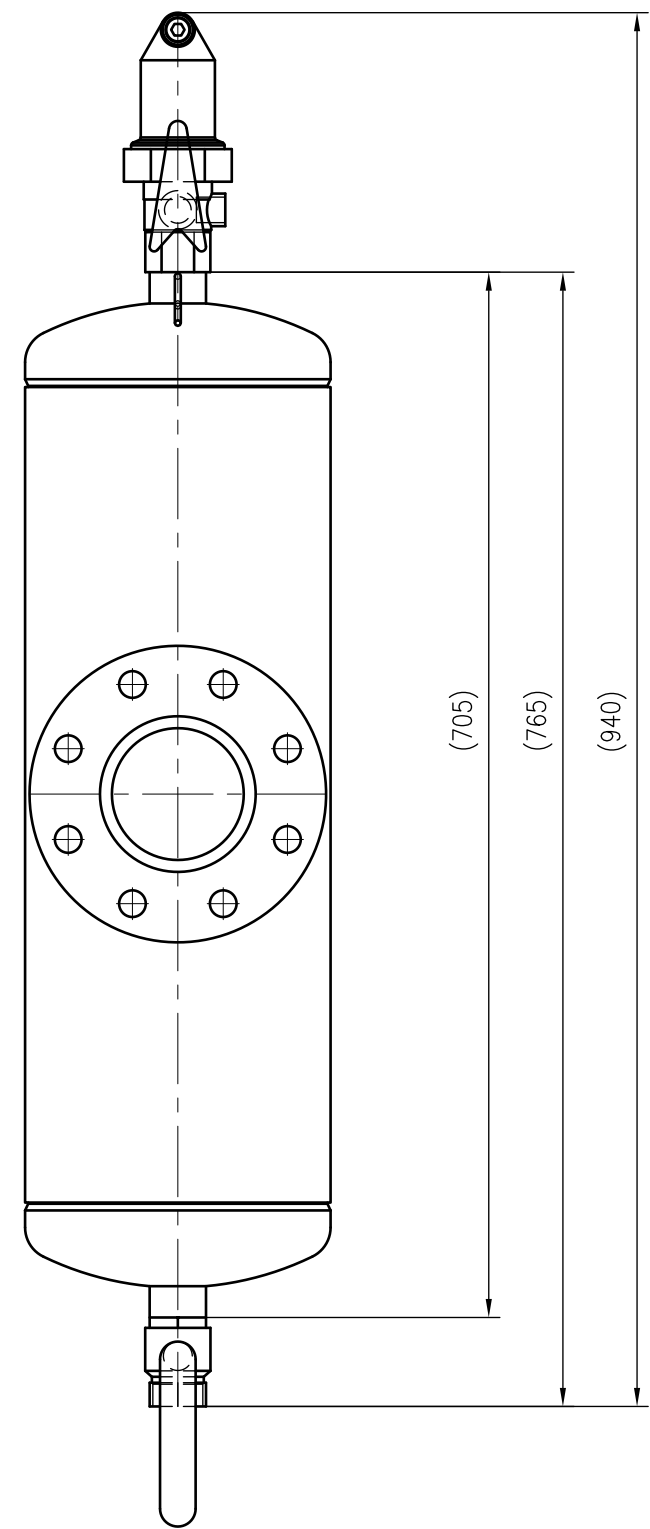
Side view
