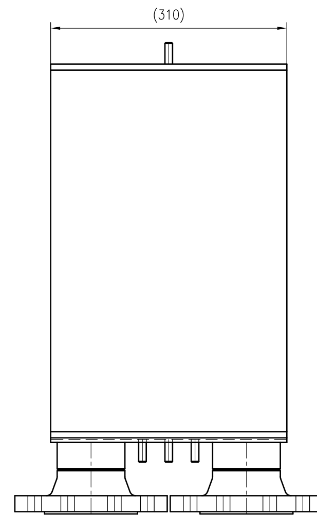
Top view
