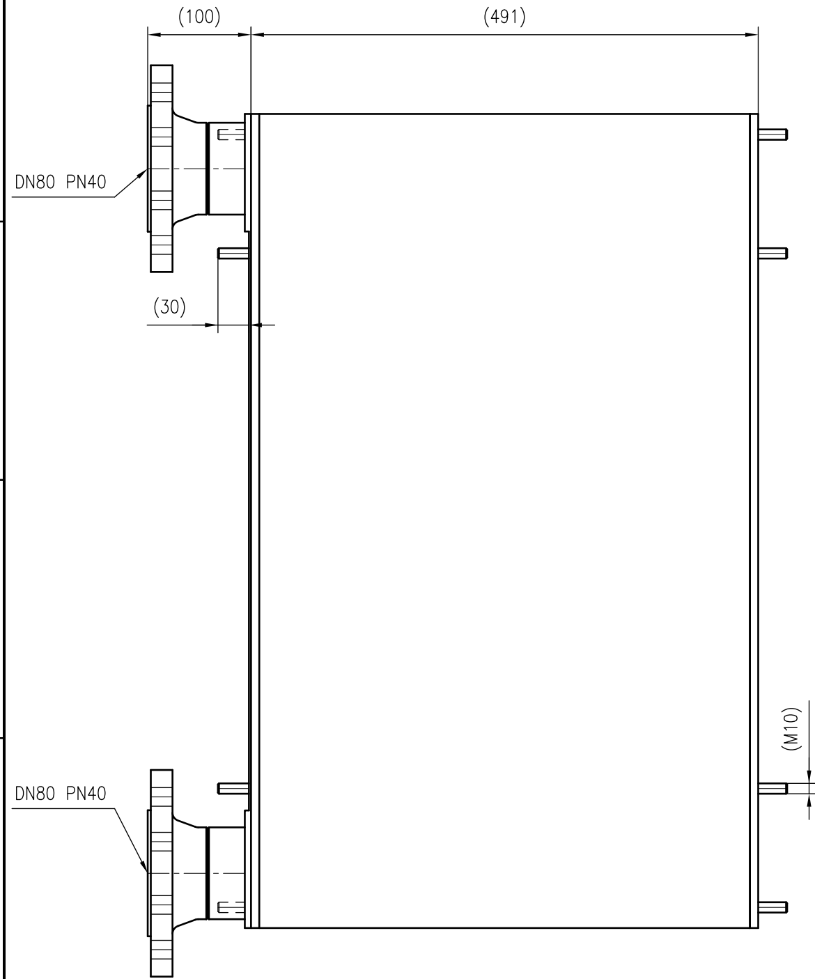
Side view
