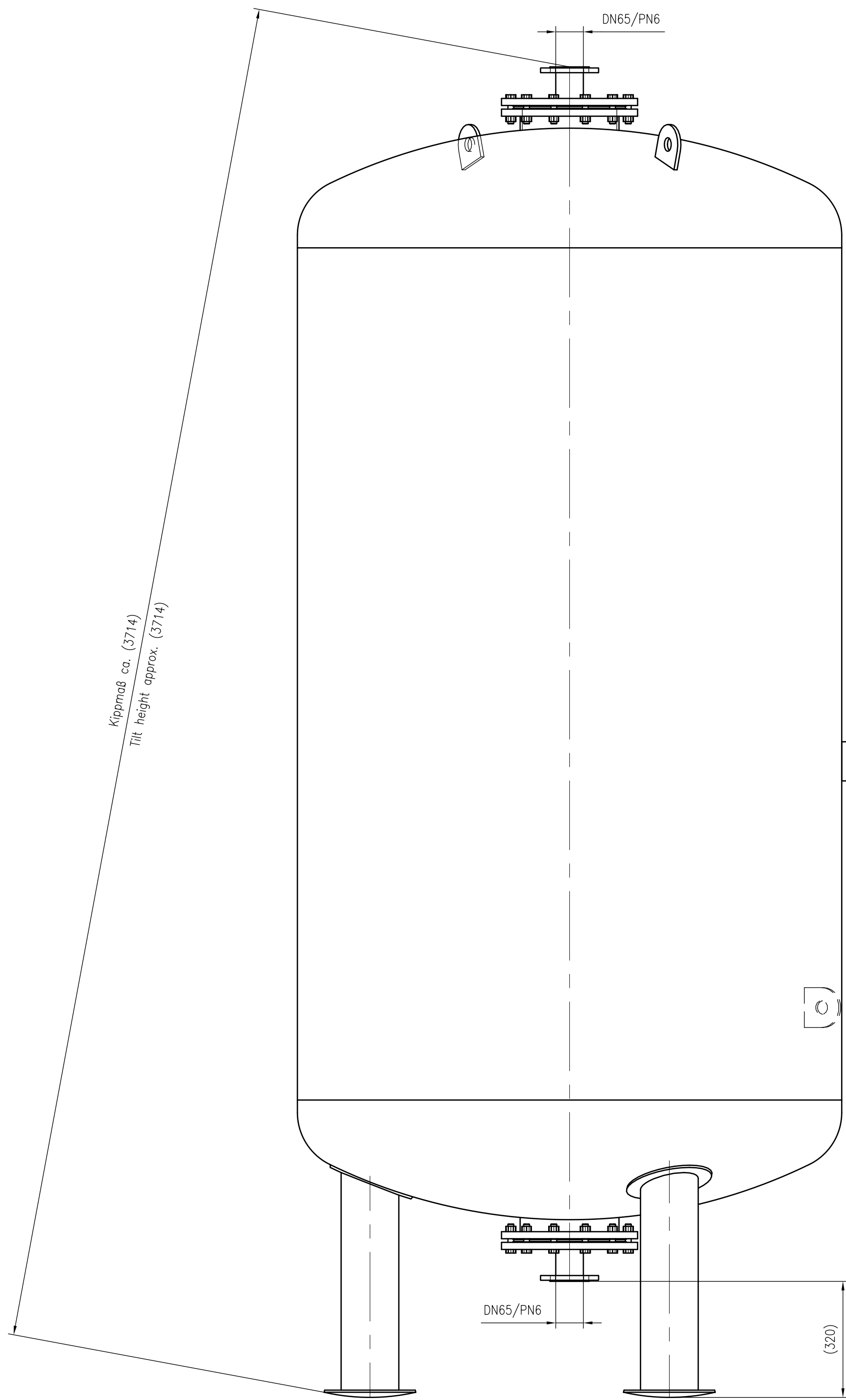
Side view
