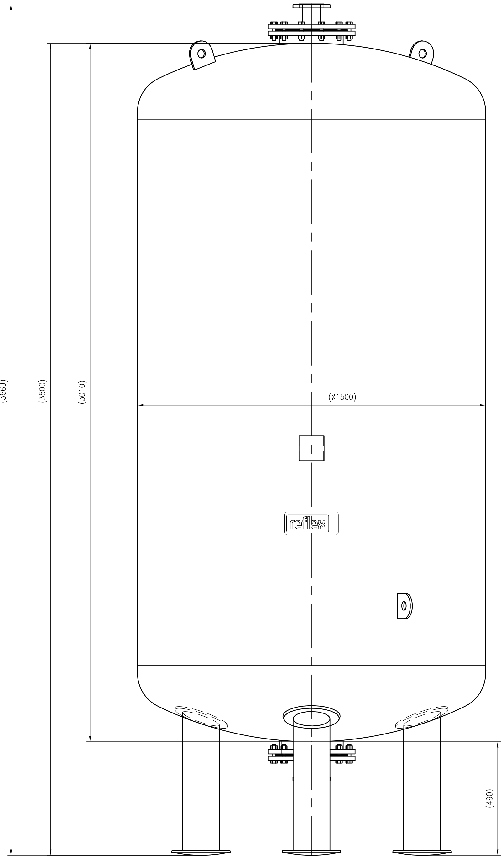
Front view
