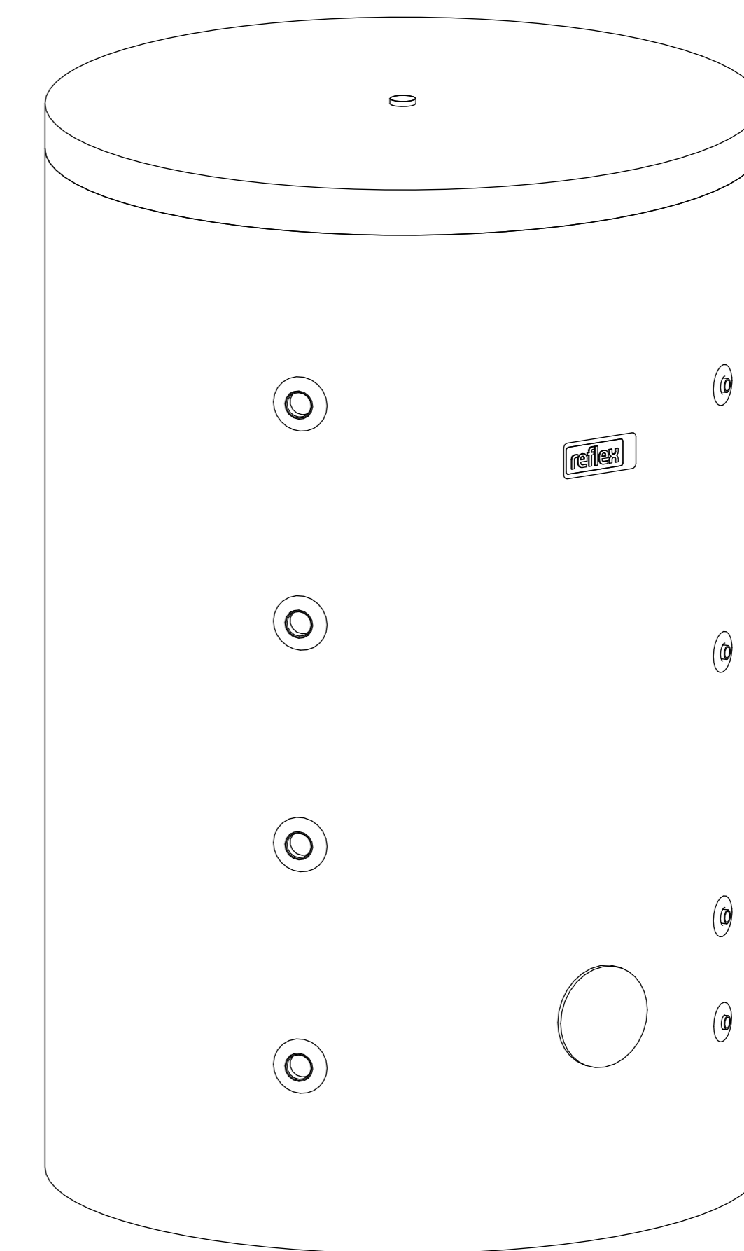
Isometric view
