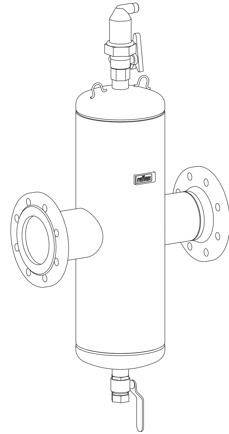
Isometric view
