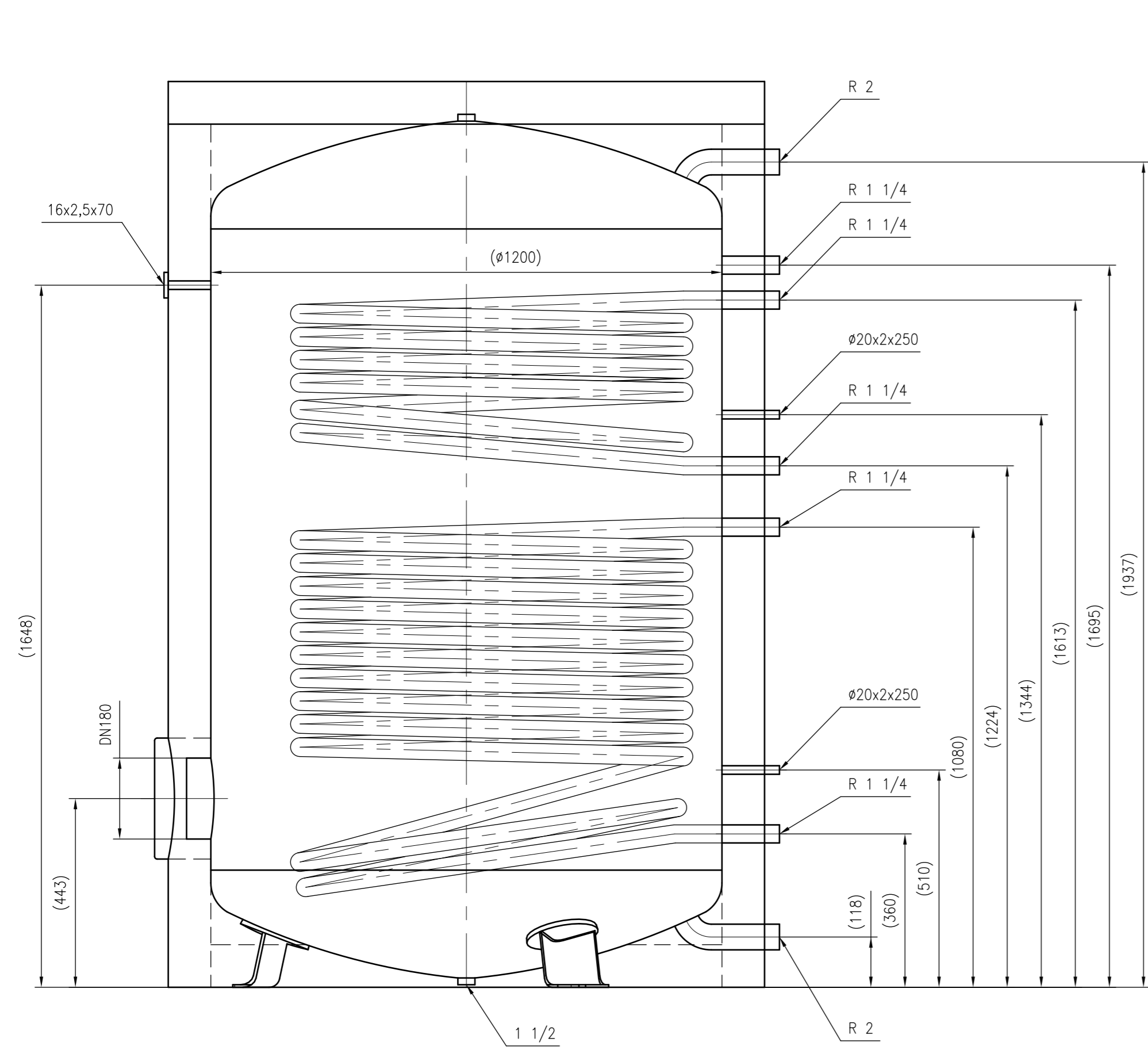
Side view
