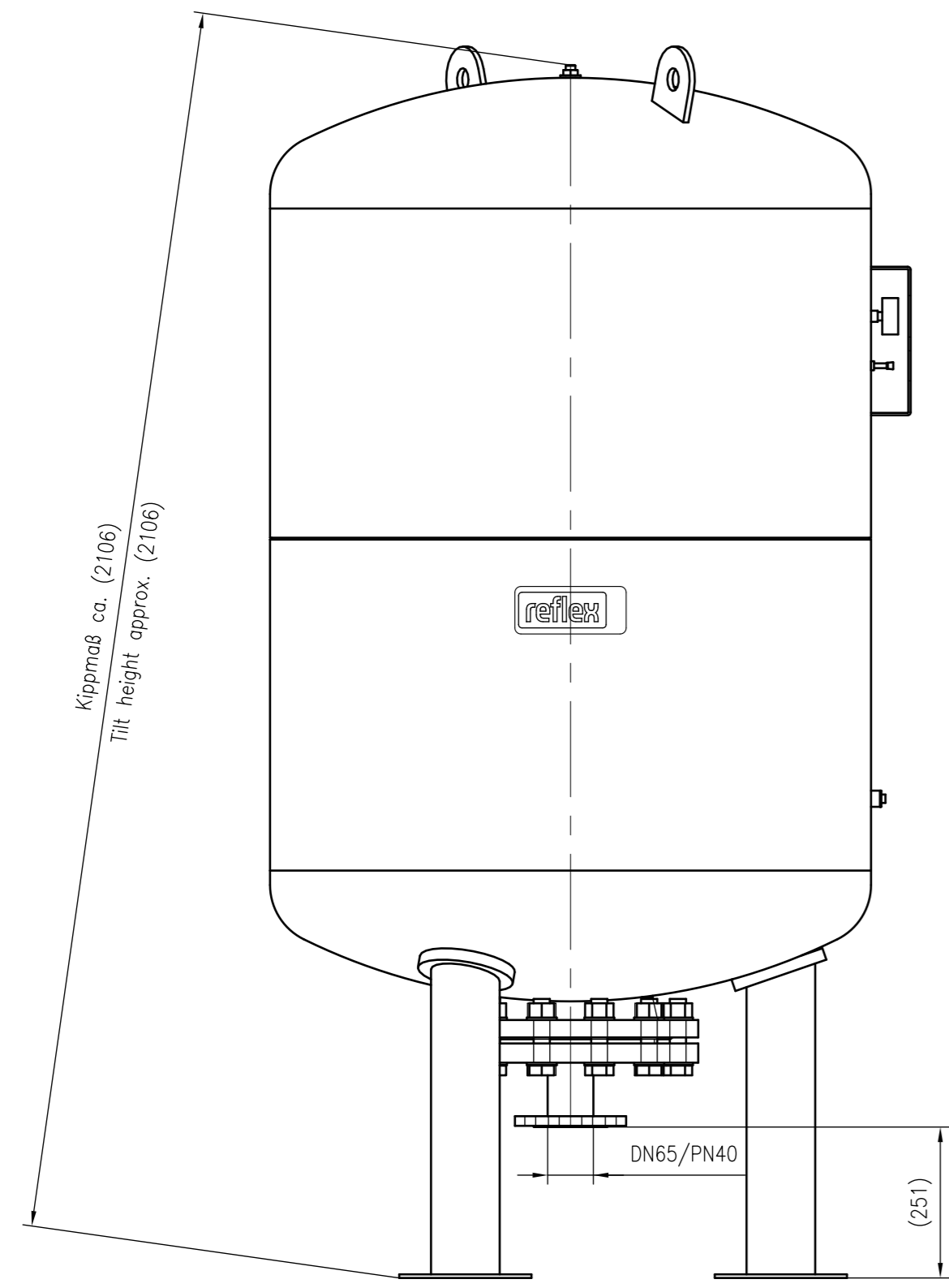
Side view
