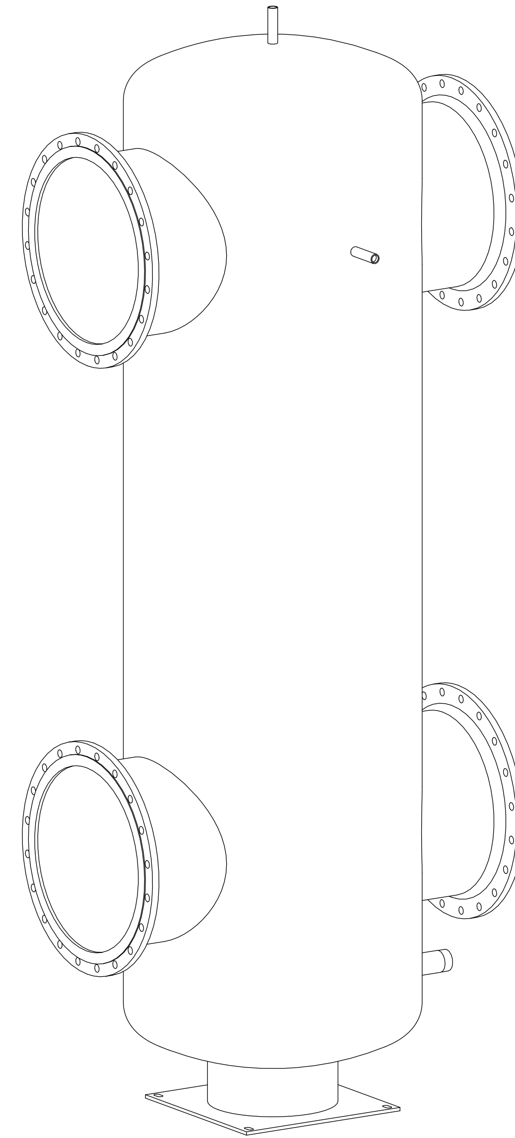
Isometric view
