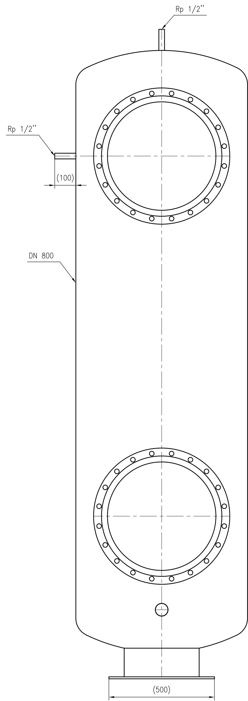
Side view
