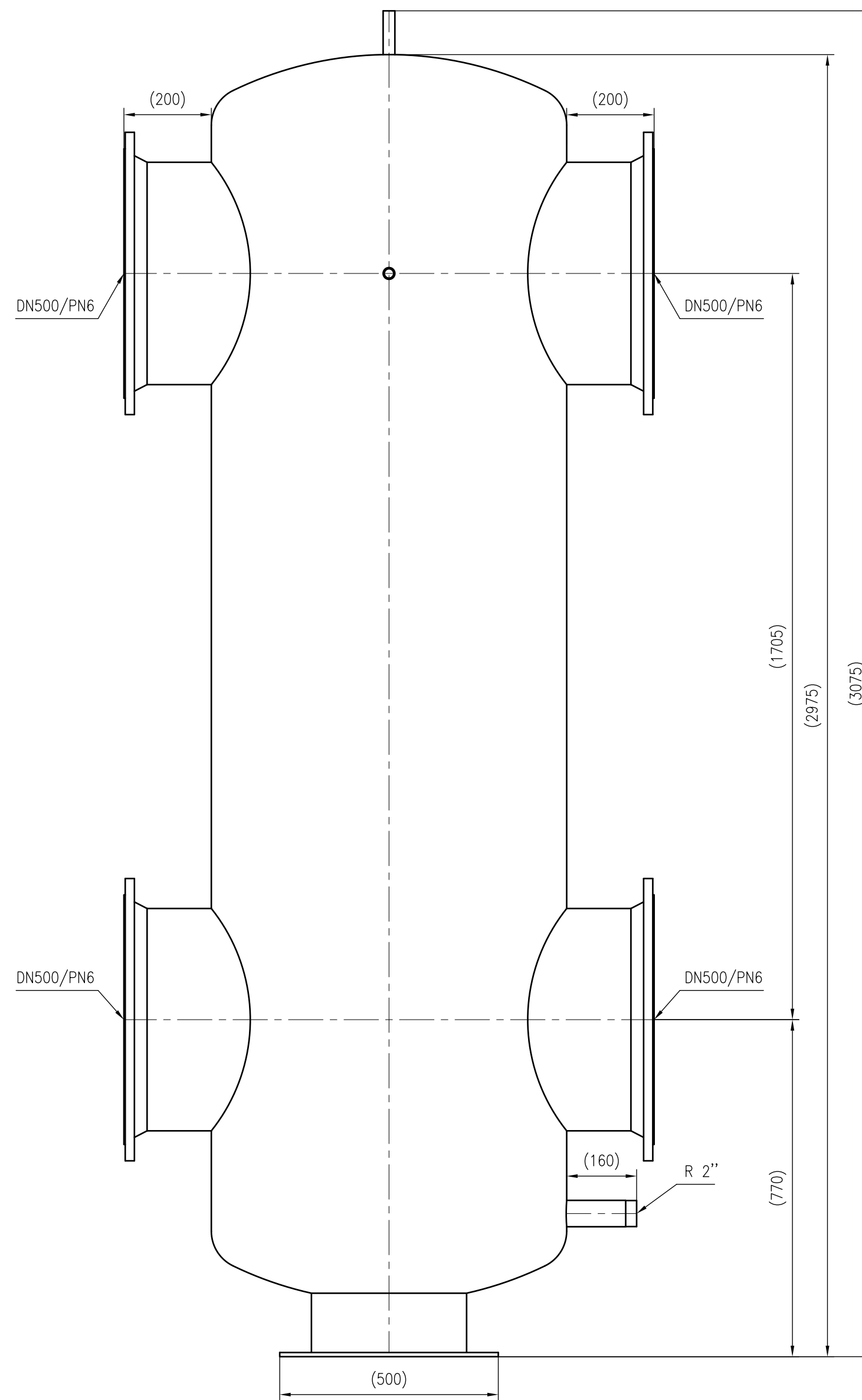
Front view
