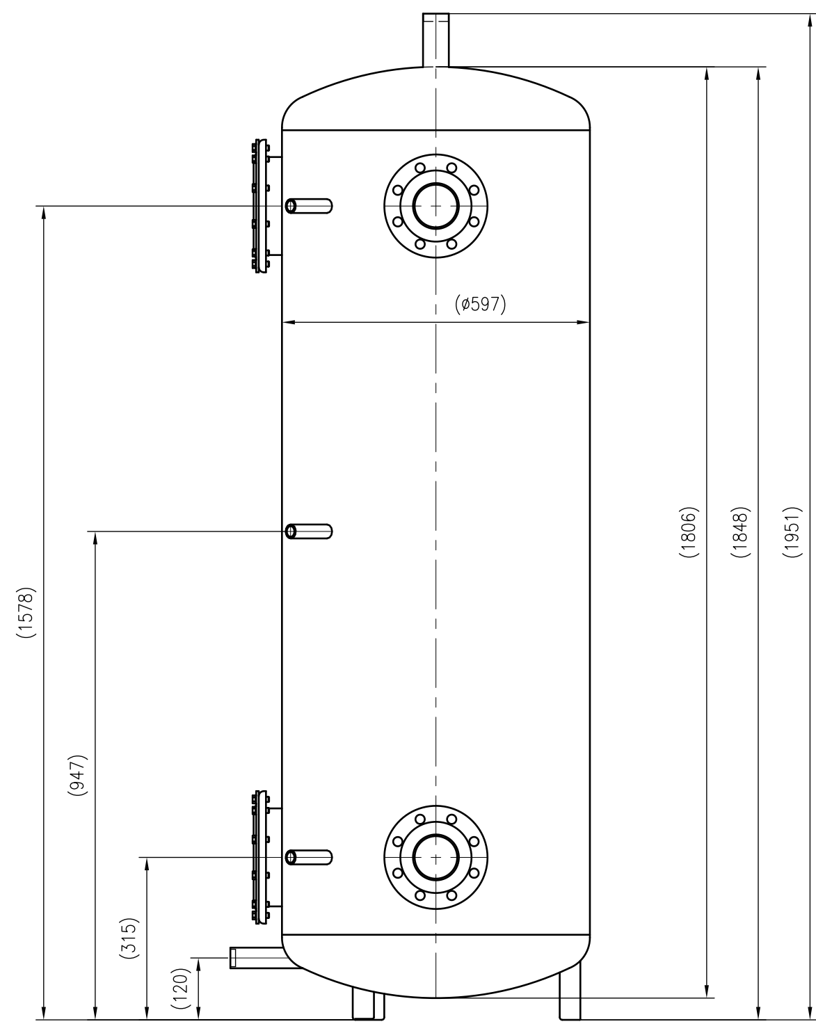
Side view
