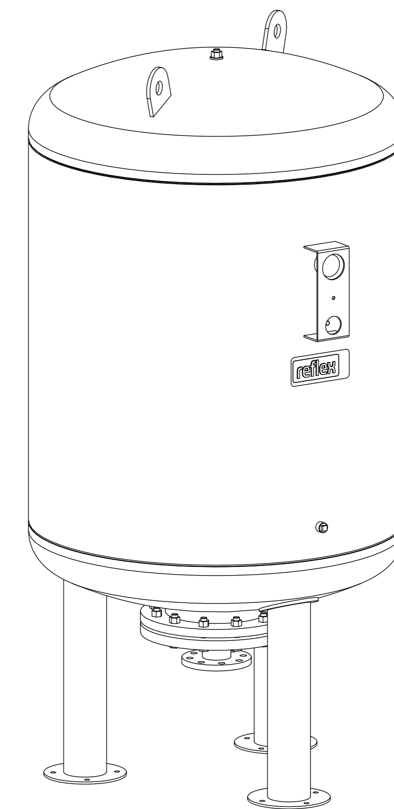
Isometric view
