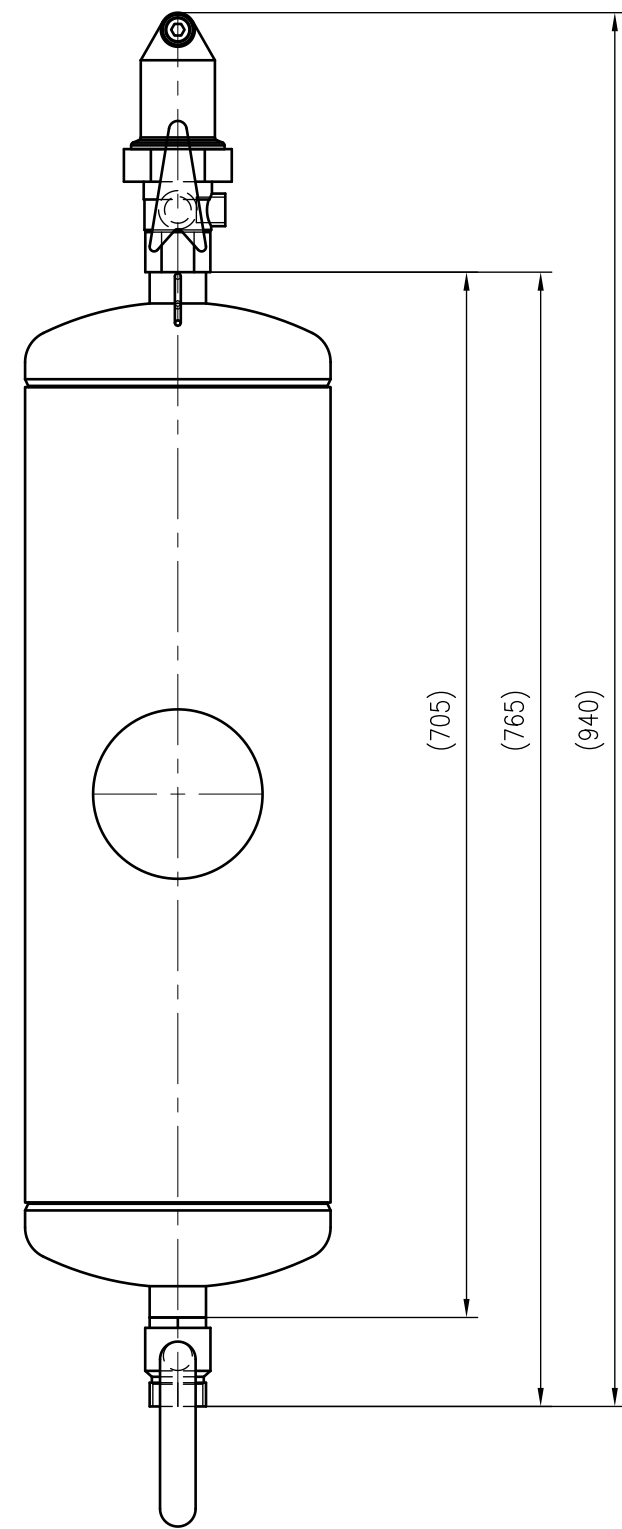
Side view
