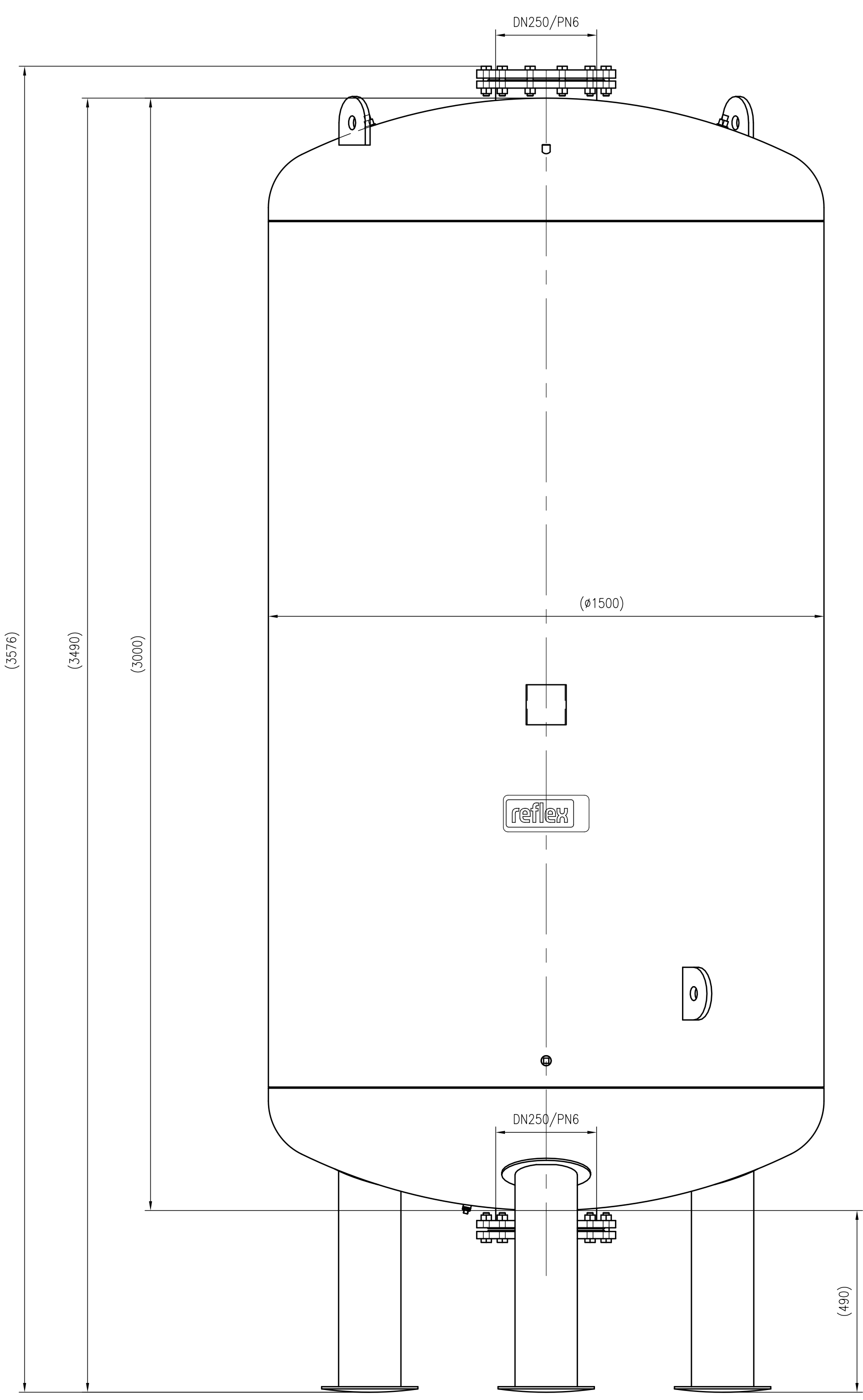
Front view
