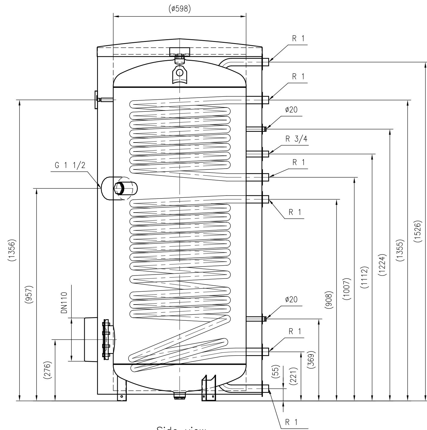
Side view
