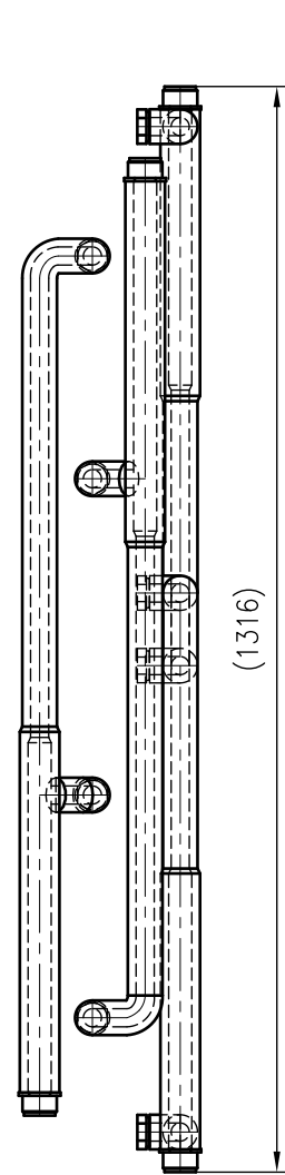
Side view
