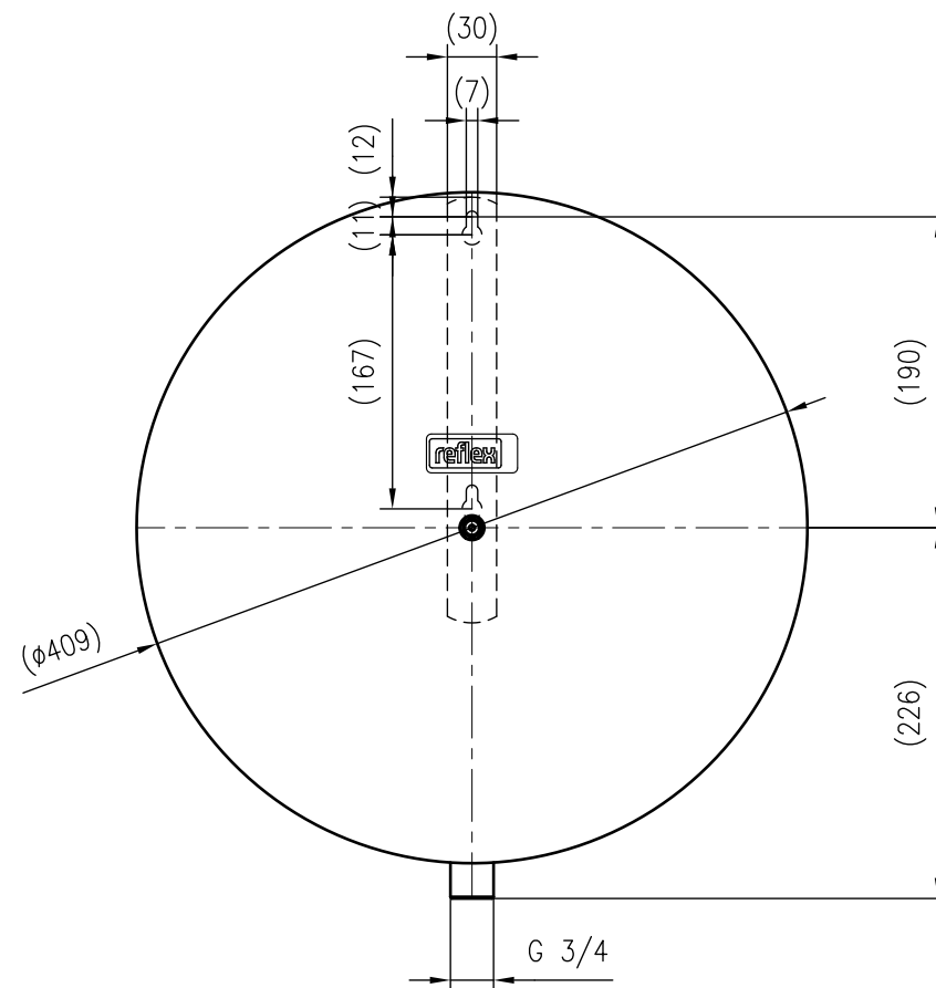
Front view
