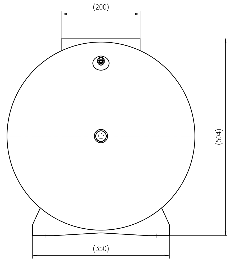
Side view
