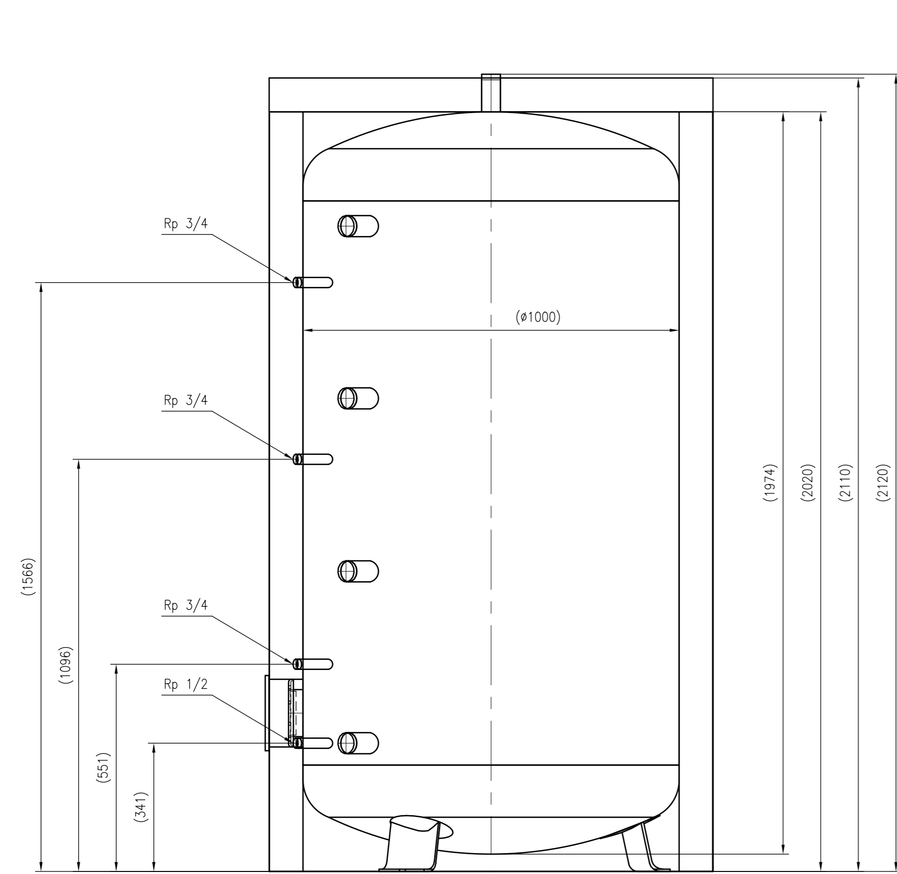
Side view
